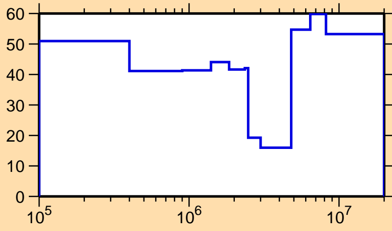
\Delta\sigma/\sigma vs. E for ^{139}\text{Eu}(n,n_1)
