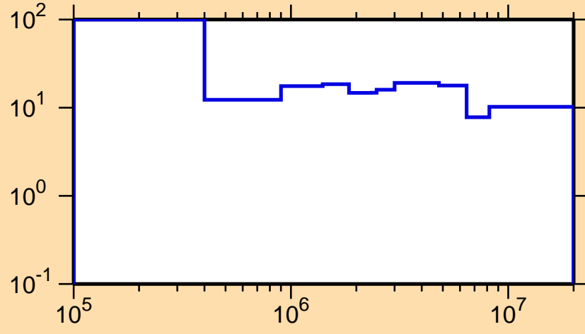
\Delta\sigma/\sigma vs. E for ^{139}\text{Eu}(n,\text{el.})
