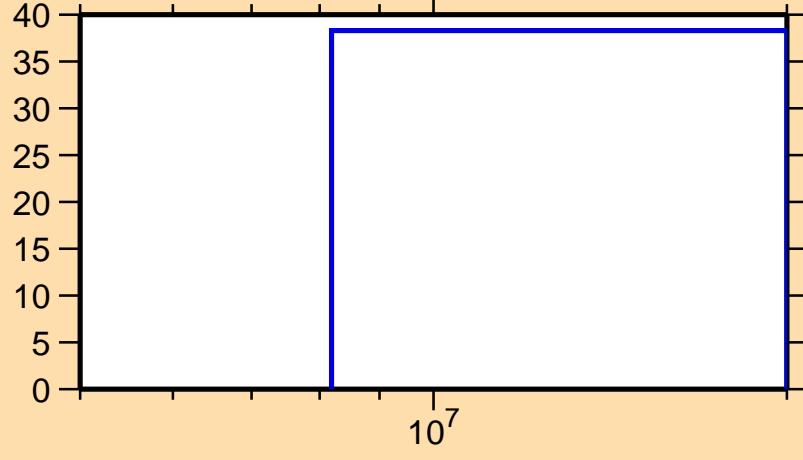
\Delta\sigma/\sigma vs. E for ^{139}\text{Eu}(n,\text{inel.})
