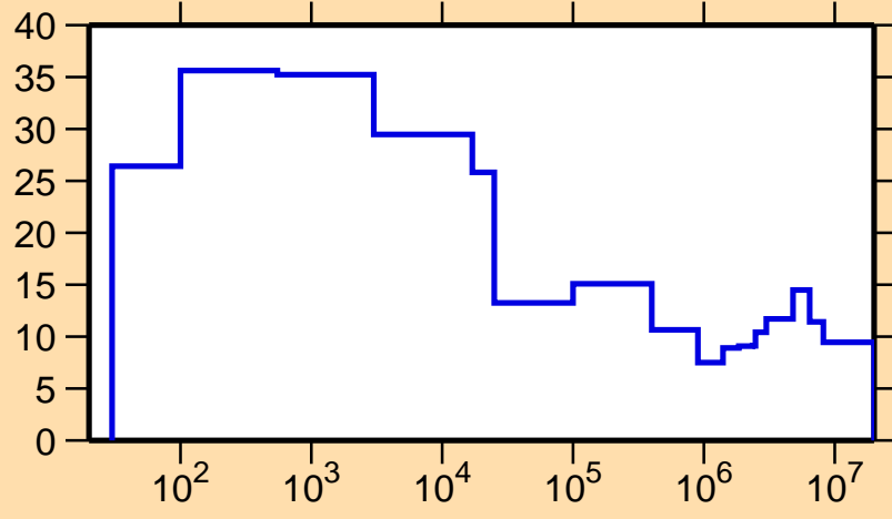
\Delta\sigma/\sigma vs. E for ^{139}\text{Eu}(n,\text{nonel.})
