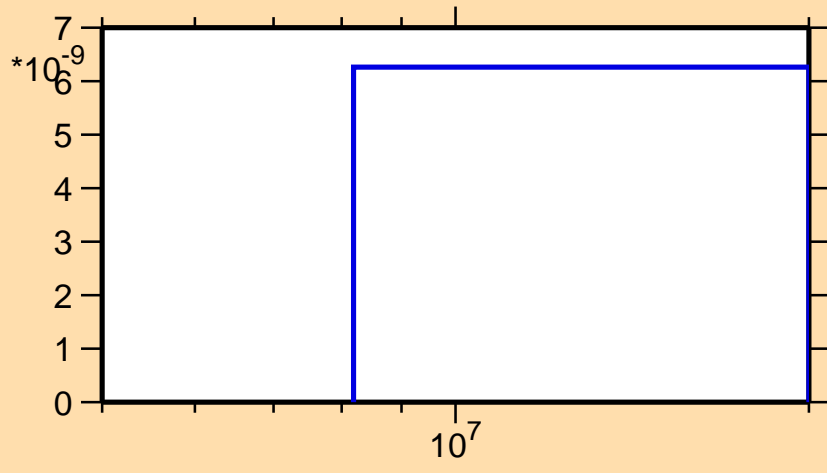
\sigma vs. E for ^{139}\text{Eu}(n,2n\alpha)
