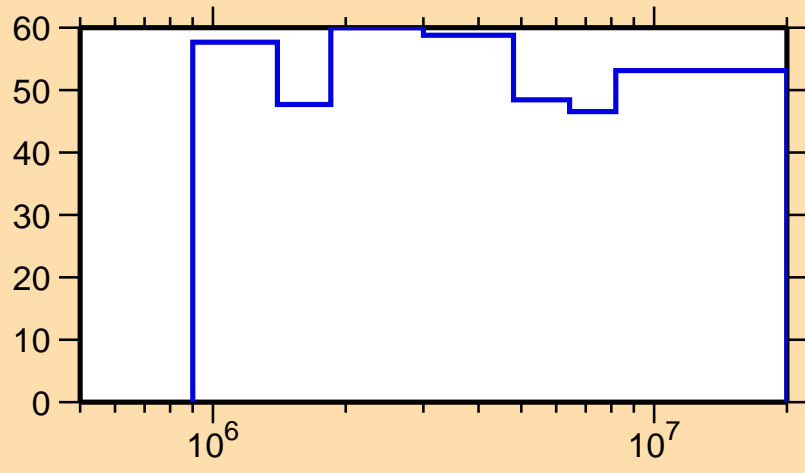
\Delta\sigma/\sigma vs. E for ^{139}\text{Eu}(n,n\text{cont.})
