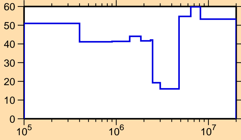
\Delta\sigma/\sigma vs. E for ^{139}\text{Eu}(n,n_1)
