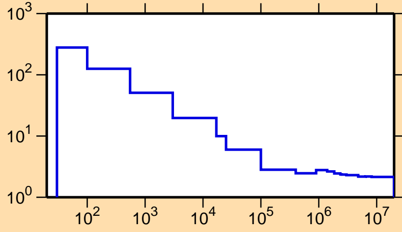
\sigma vs. E for ^{139}\text{Eu}(n,\text{nonel.})
