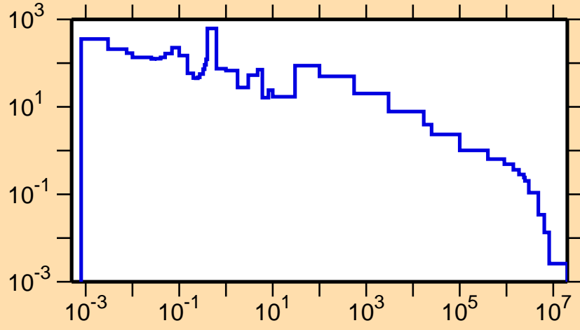
\sigma vs. E for ^{139}\text{Eu}(n,\gamma)
