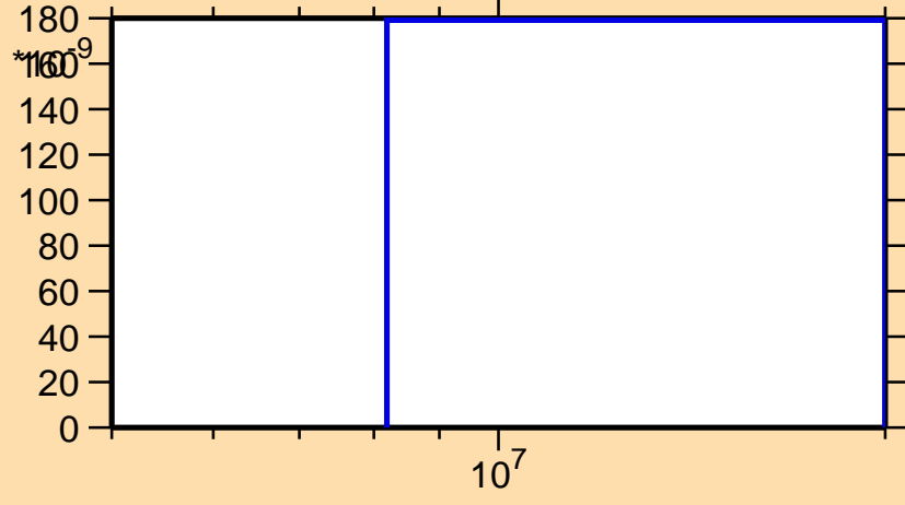
\sigma vs. E for ^{139}\text{Eu}(n,\text{nd})
