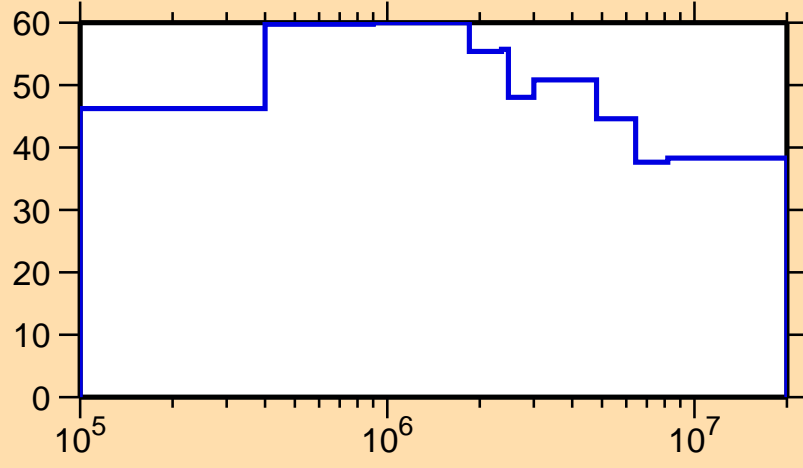
\Delta\sigma/\sigma vs. E for ^{139}\text{Eu}(n,\text{inel.})
