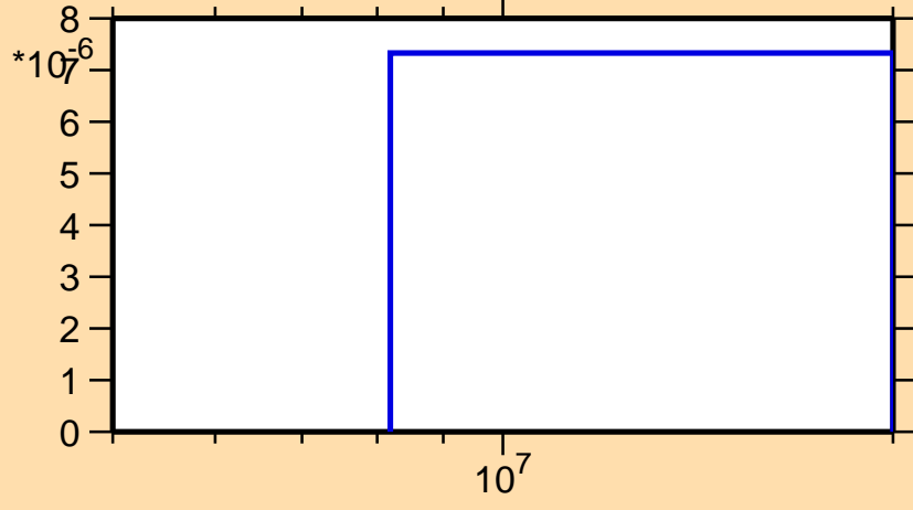
\sigma vs. E for ^{139}\text{Eu}(n,\text{pd})
