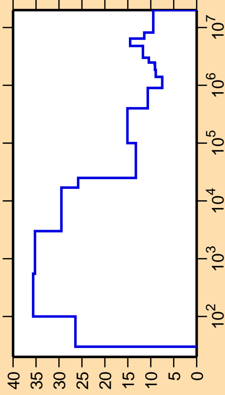
\Delta\sigma/\sigma vs. E for ^{139}\text{Eu}(n,\text{nonel.})
