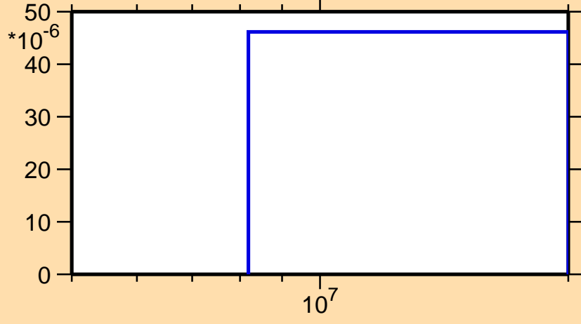
\sigma vs. E for ^{139}\text{Eu}(n,2np)
