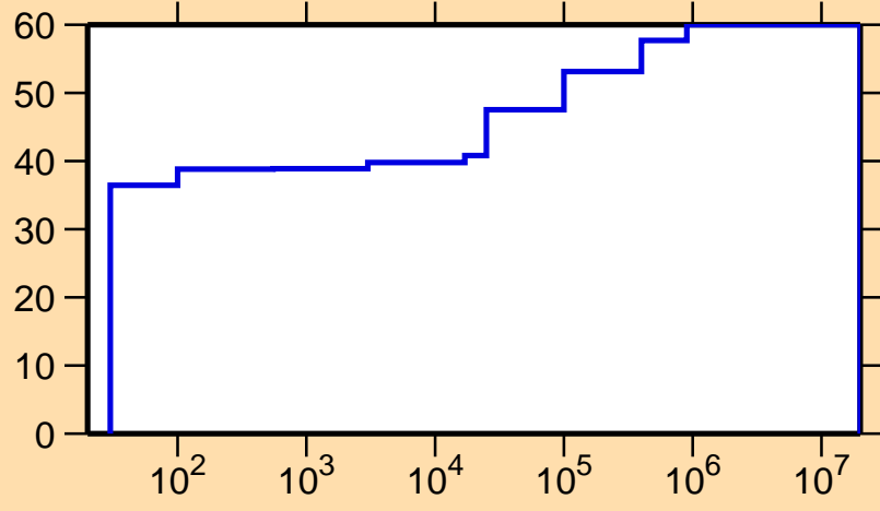
\Delta\sigma/\sigma vs. E for ^{139}\text{Eu}(n,\gamma)
