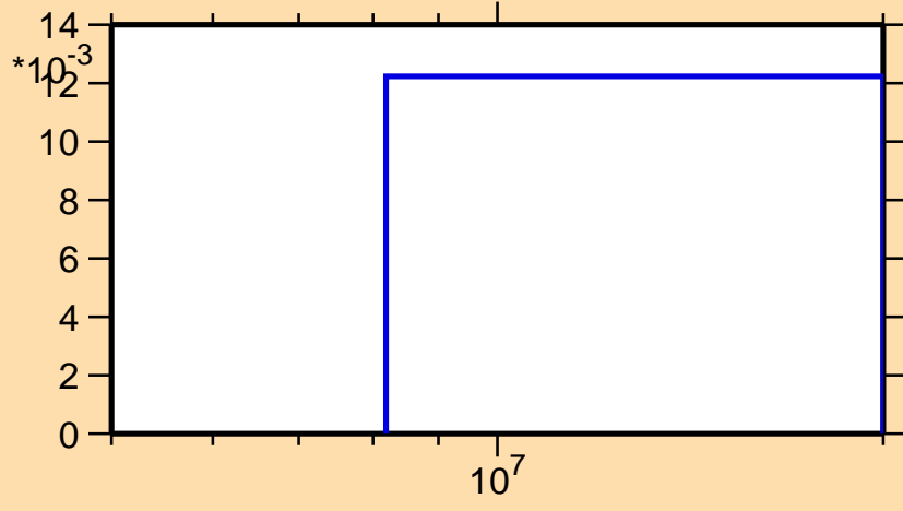
\sigma vs. E for ^{139}\text{Eu}(n,2n)
