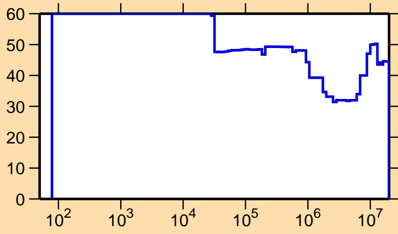
\Delta\sigma/\sigma vs. E for ^{140}\text{Eu}(n,p)
