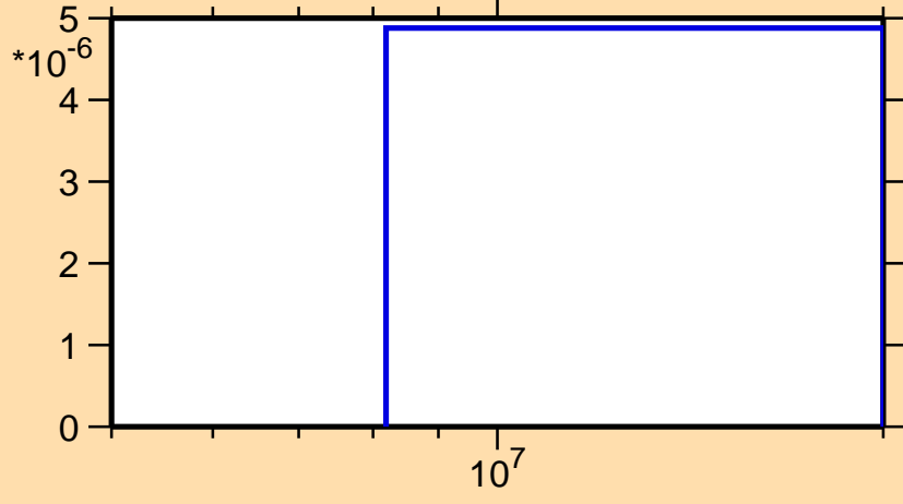
\sigma vs. E for ^{140}\text{Eu}(n,\text{nd})
