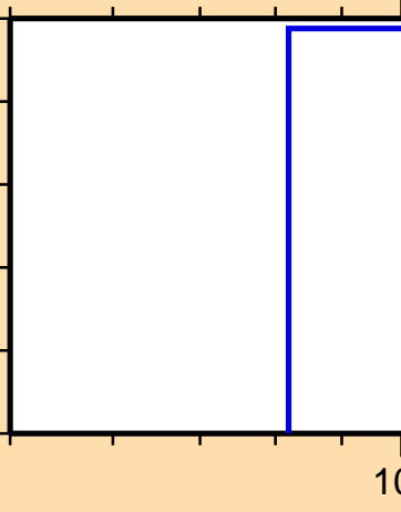
\sigma vs. E for ^{140}\text{Eu}(n,\text{nd})
