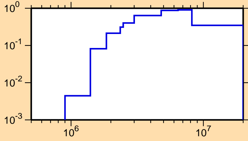
\sigma vs. E for ^{140}\text{Eu}(n,n\text{cont.})
