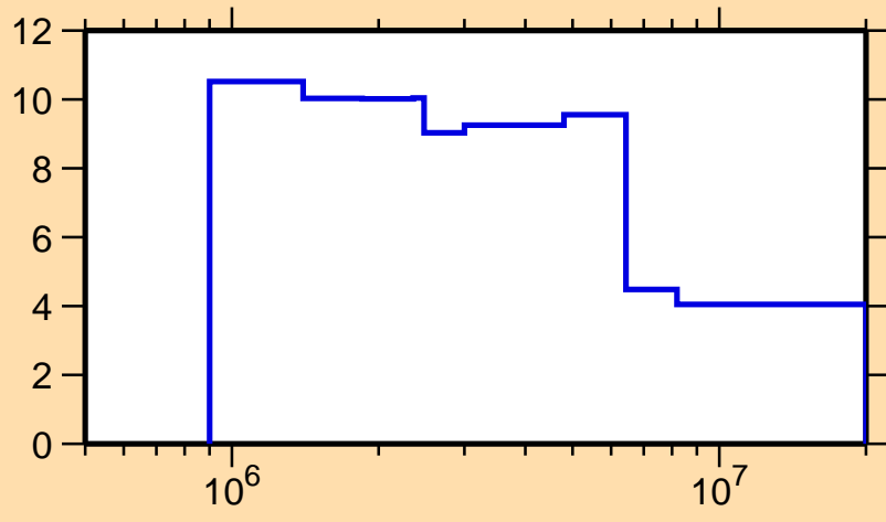
\Delta\sigma/\sigma vs. E for ^{140}\text{Eu}(n, tot.)
