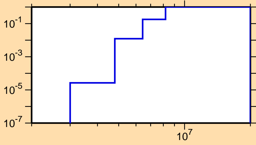
\sigma vs. E for ^{140}\text{Eu}(n,np)
