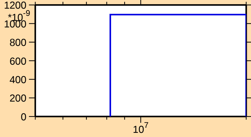
\sigma vs. E for ^{141}\text{Eu}(n,\text{pd})
