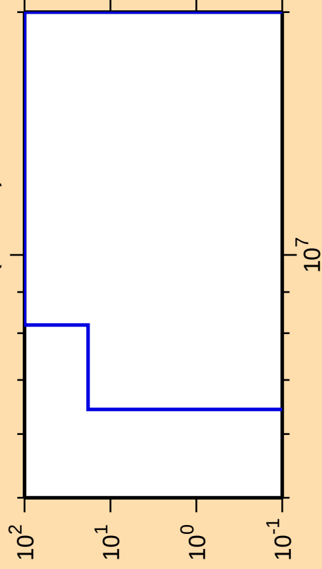
\Delta\sigma/\sigma vs. E for ^{141}\text{Eu}(n,\text{He3})
