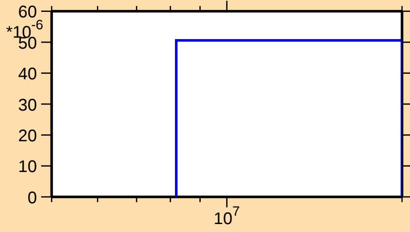
\sigma vs. E for ^{141}\text{Eu}(n,2np)
