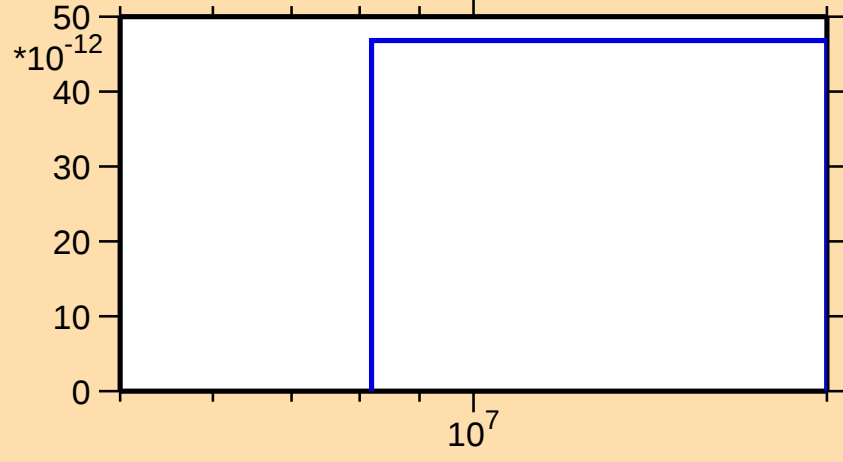
\sigma vs. E for ^{141}\text{Eu}(n,nt)
