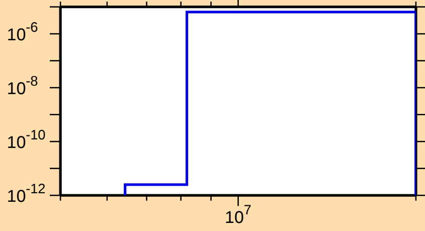
\sigma vs. E for ^{141}\text{Eu}(n,\text{He3})
