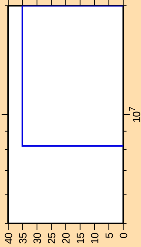
\Delta\sigma/\sigma vs. E for ^{141}\text{Eu}(n,n_1)
