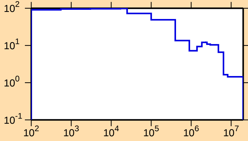
\Delta\sigma/\sigma vs. E for ^{141}\text{Eu}(n,\text{tot.})
