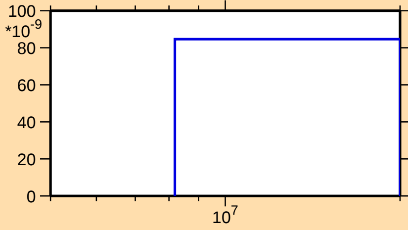
\sigma vs. E for ^{141}\text{Eu}(\text{mt117})
