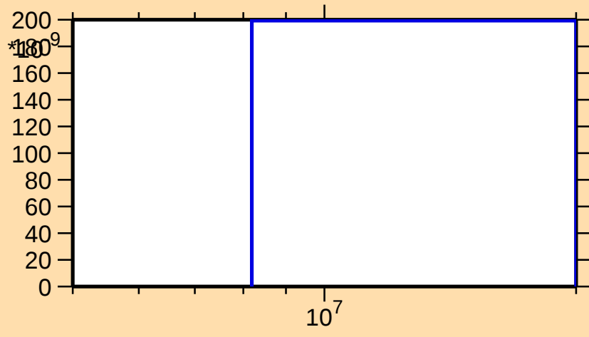
\sigma vs. E for ^{141}\text{Eu}(n,nd)
