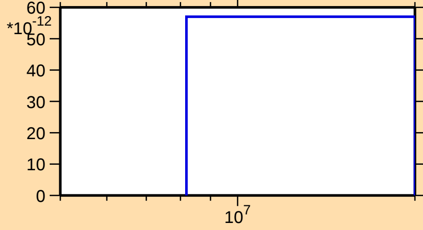
\sigma vs. E for ^{141}\text{Eu}(n,pt)
