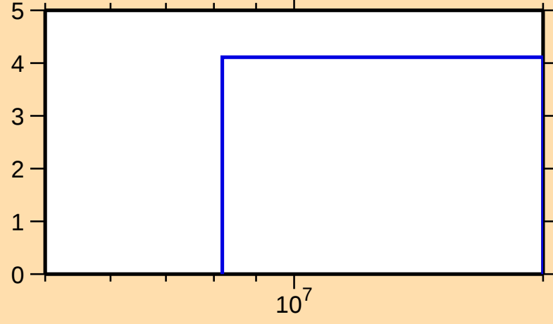
\Delta\sigma/\sigma vs. E for ^{141}\text{Eu}(n,\text{el.})
