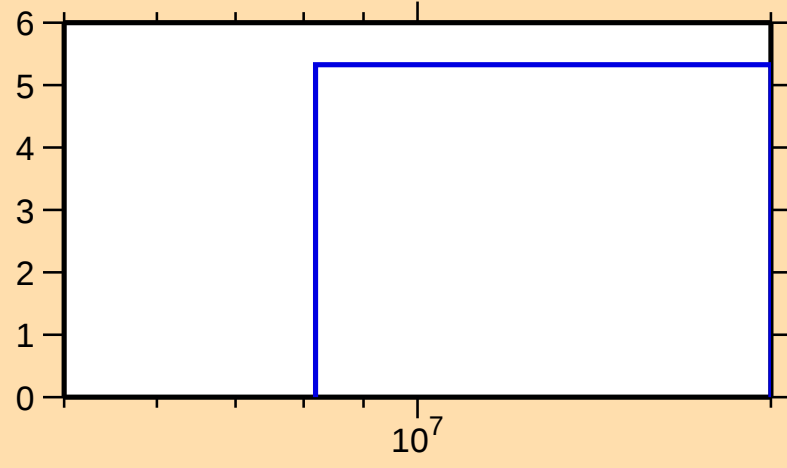
\Delta\sigma/\sigma vs. E for ^{141}\text{Eu}(n,\text{nonel.})
