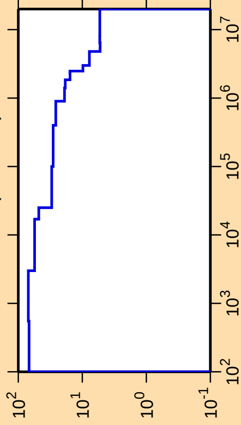
\Delta\sigma/\sigma vs. E for ^{141}\text{Eu}(n,\text{nonel.})
