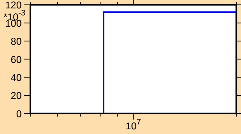
\sigma vs. E for ^{141}\text{Eu}(n,2n)
