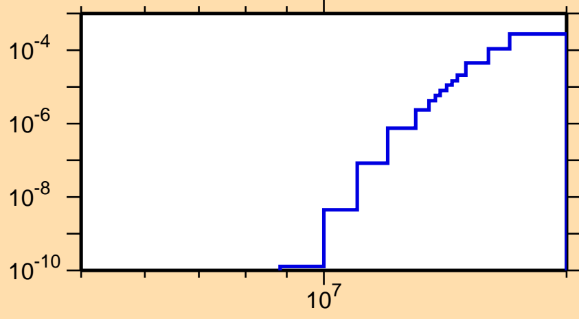
\sigma vs. E for ^{141}\text{Eu}(\text{mt } 45)
