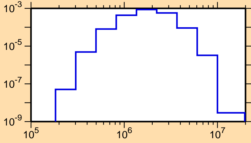
\sigma vs. E for ^{141}\text{Eu}(n,n_4)
