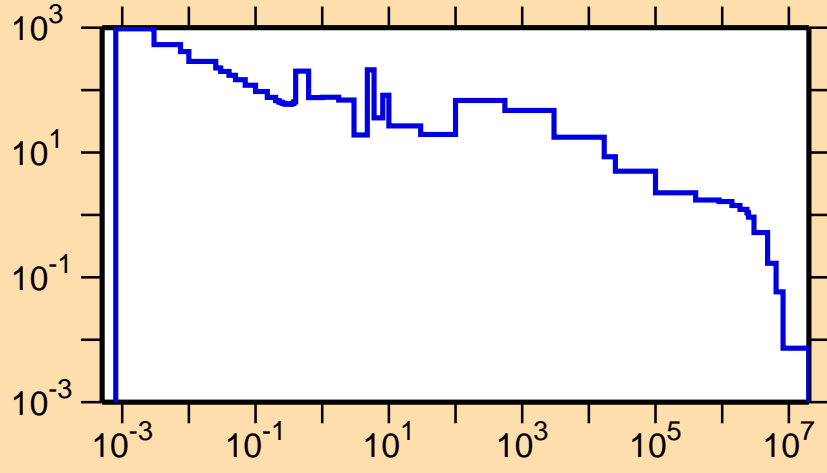
\sigma vs. E for ^{141}\text{Eu}(n,\gamma)
