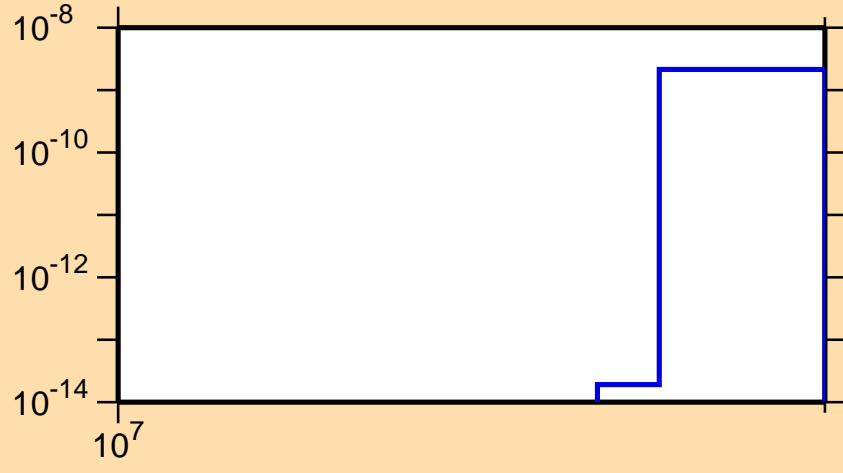
\sigma vs. E for ^{142}\text{Eu}(n,nt)
