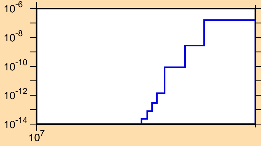
\sigma vs. E for ^{142}\text{Eu}(n,pt)
