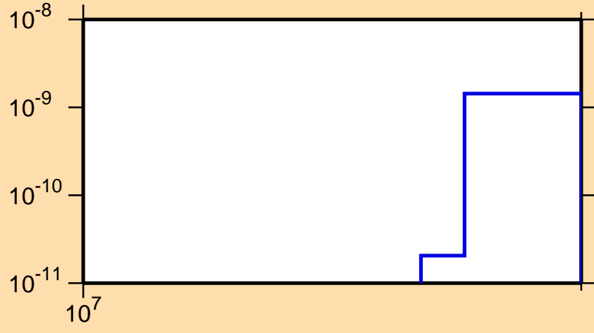
\sigma vs. E for ^{142}\text{Eu} (mt 34)
