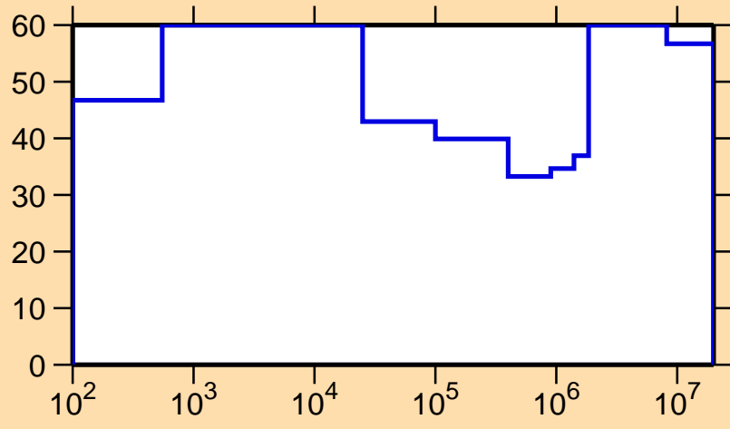
\Delta\sigma/\sigma vs. E for ^{142}\text{Eu}(n,p)
