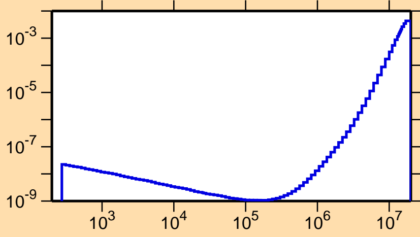
\sigma vs. E for ^{142}\text{Eu}(n,p\alpha)
