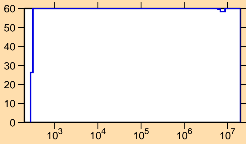
\Delta\sigma/\sigma vs. E for ^{142}\text{Eu}(n,n\text{cont.})
