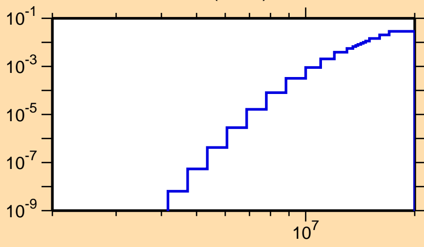
\sigma vs. E for ^{142}\text{Eu}(n,n\alpha)
