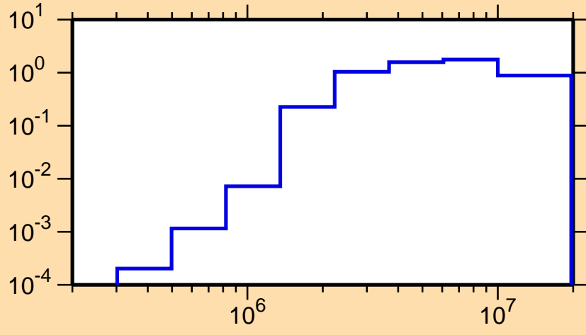
\sigma vs. E for ^{142}\text{Eu}(n,n\text{cont.})
