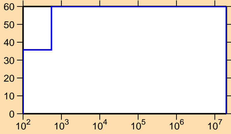
\Delta\sigma/\sigma vs. E for ^{142}\text{Eu}(n,\gamma)
