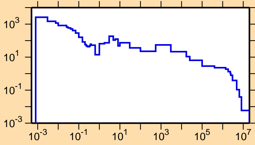
\sigma vs. E for ^{142}\text{Eu}(n,\gamma)
