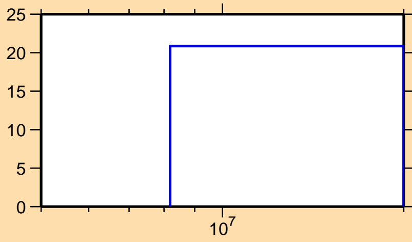
\Delta\sigma/\sigma vs. E for ^{142}\text{Eu}(n,\text{el.})
