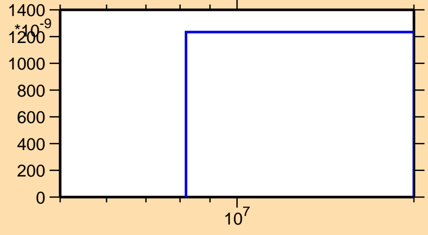
\sigma vs. E for ^{142}\text{Eu} (mt 45)
