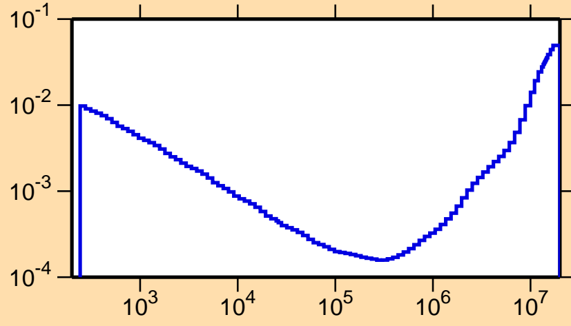
\sigma vs. E for ^{143}\text{Eu}(n,\alpha)
