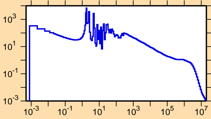
\sigma vs. E for ^{143}\text{Eu}(n,\gamma)
