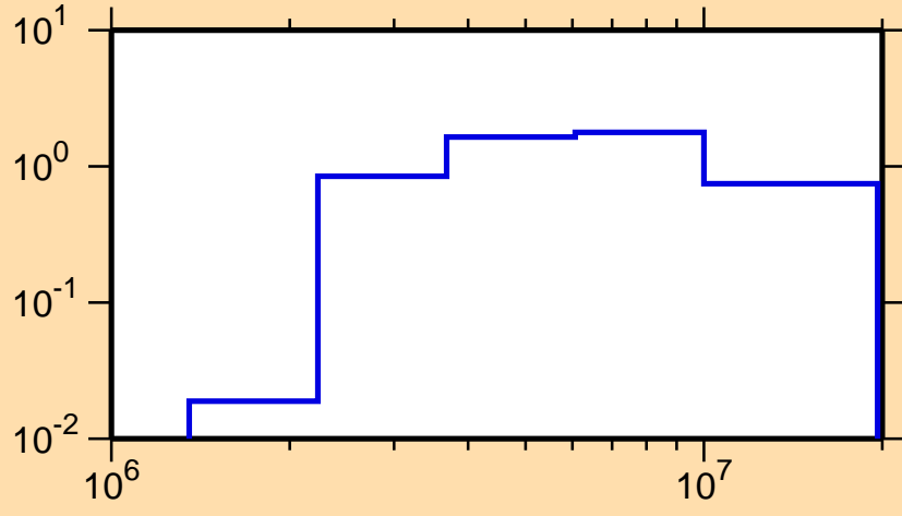
\sigma vs. E for ^{143}\text{Eu}(n,n\text{cont.})
