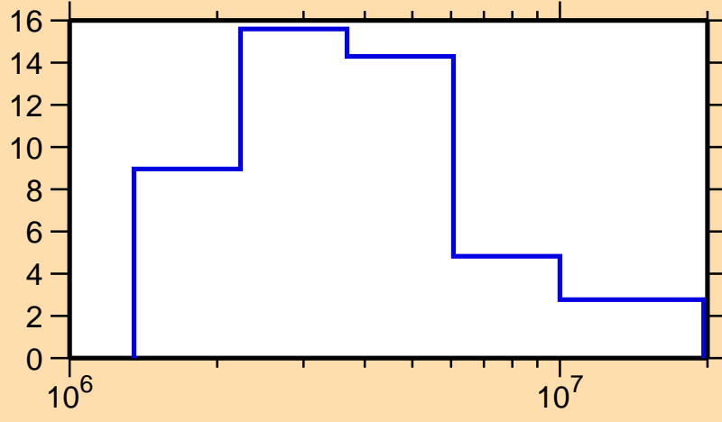
\Delta\sigma/\sigma vs. E for ^{143}\text{Eu}(n, el.)
