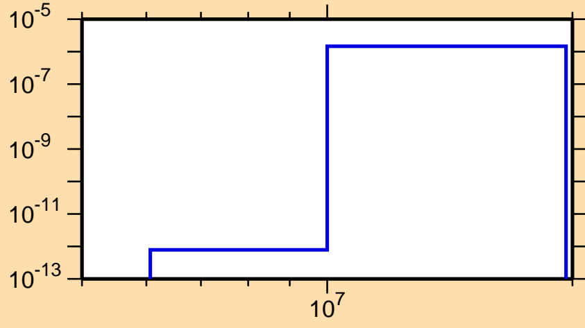
\sigma vs. E for ^{143}\text{Eu}(n,\text{He3})
