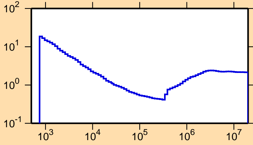
\sigma vs. E for ^{145}\text{Eu}(n,\text{nonel.})
