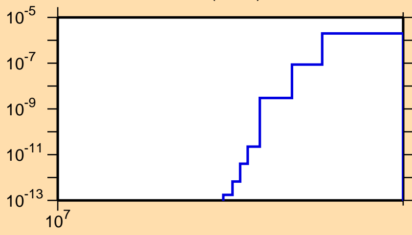
\sigma vs. E for ^{145}\text{Eu}(n,nd)
