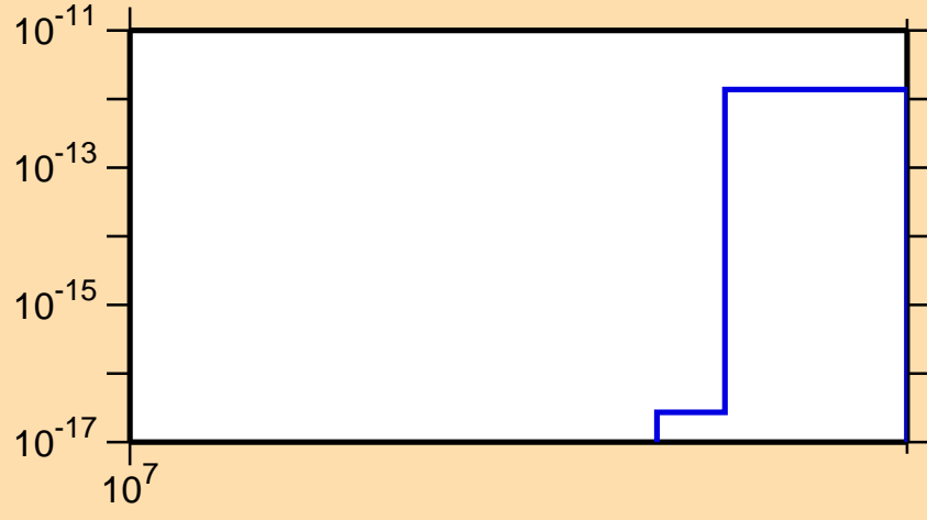
\sigma vs. E for ^{145}\text{Eu}(n,\text{pt})
