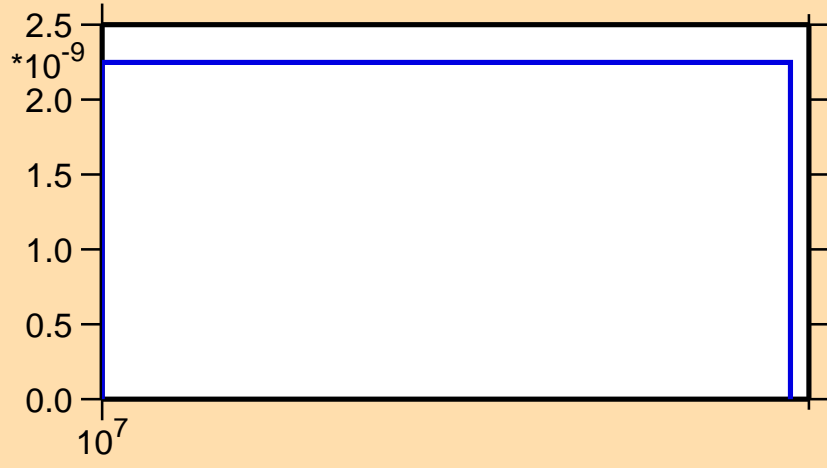
\sigma vs. E for ^{145}\text{Eu} (mt 45)
