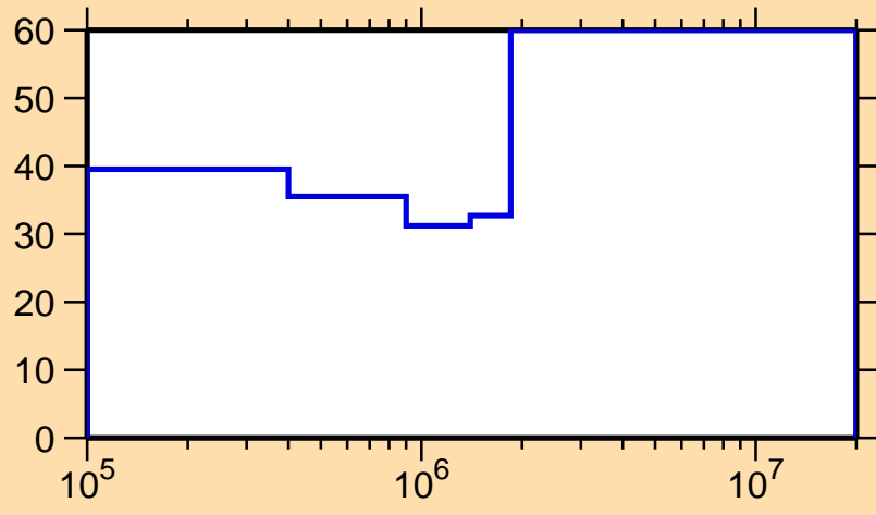
\Delta\sigma/\sigma vs. E for ^{145}\text{Eu}(n,n_1)
