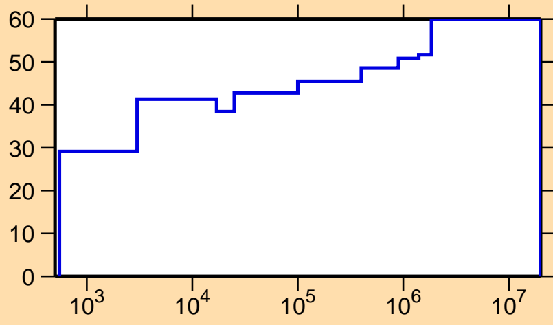
\Delta\sigma/\sigma vs. E for ^{145}\text{Eu}(n,\gamma)
