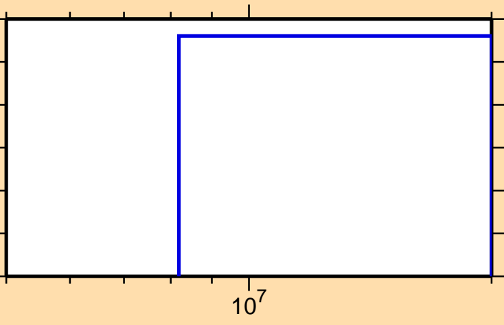
\sigma vs. E for ^{145}\text{Eu}(n,\text{pt})
