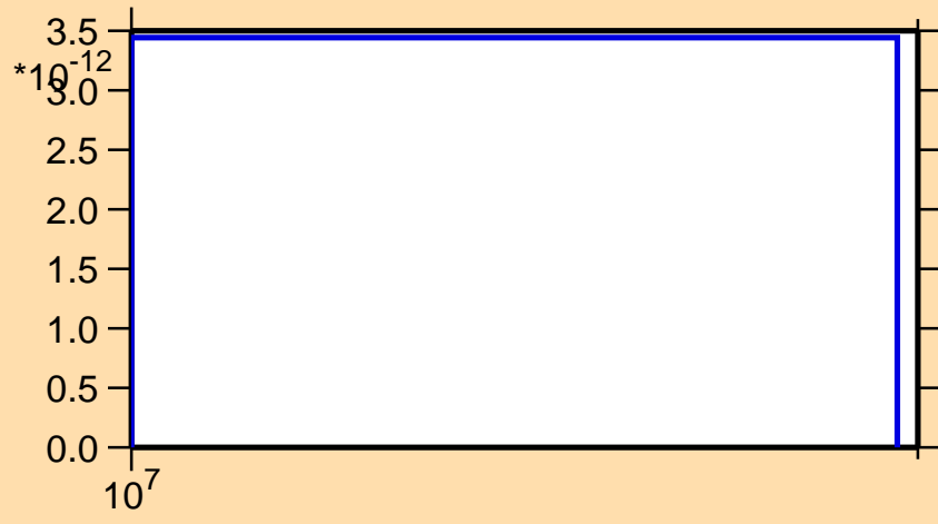
\sigma vs. E for ^{146}\text{Eu} (mt 34)
