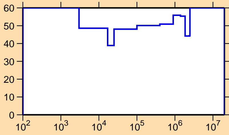
\Delta\sigma/\sigma vs. E for ^{146}\text{Eu}(n,\gamma)
