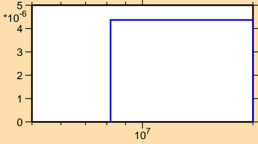
\sigma vs. E for ^{146}\text{Eu}(n,nd)
