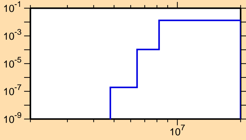
\sigma vs. E for ^{146}\text{Eu}(n,np)
