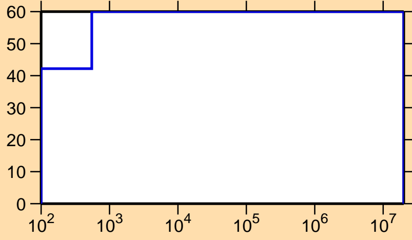
\Delta\sigma/\sigma vs. E for ^{146}\text{Eu}(n,p)
