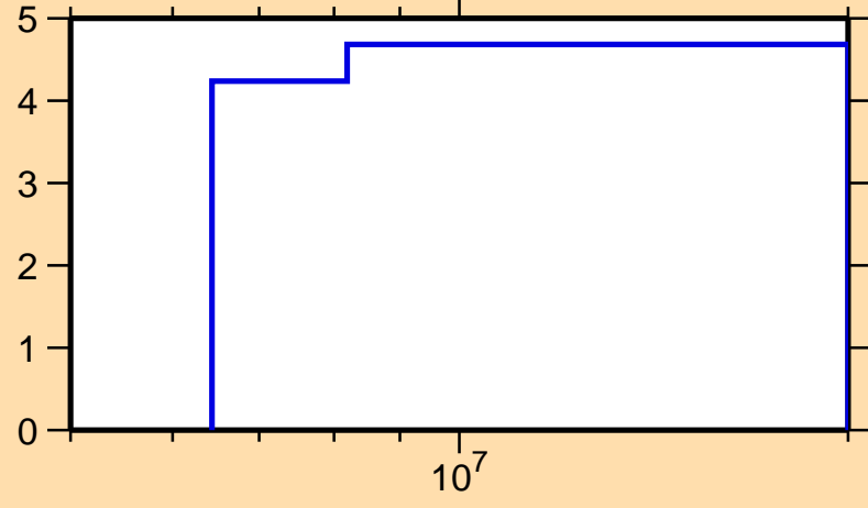
\Delta\sigma/\sigma vs. E for ^{146}\text{Eu}(n,\text{tot.})
