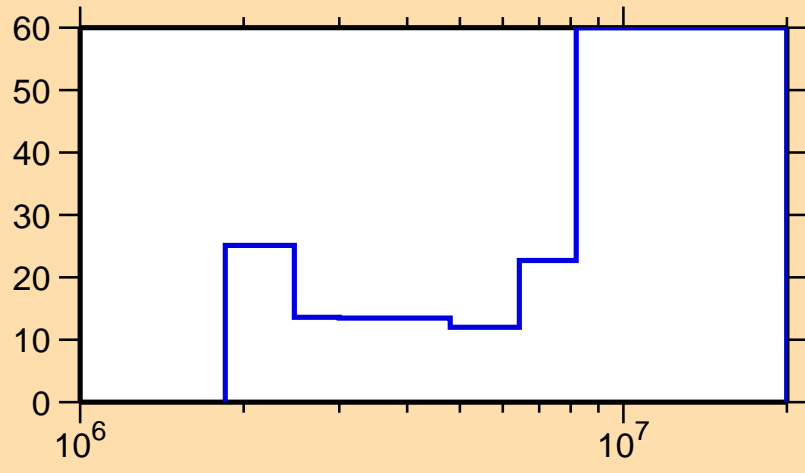
\Delta\sigma/\sigma vs. E for ^{146}\text{Eu}(n,n\text{cont.})
