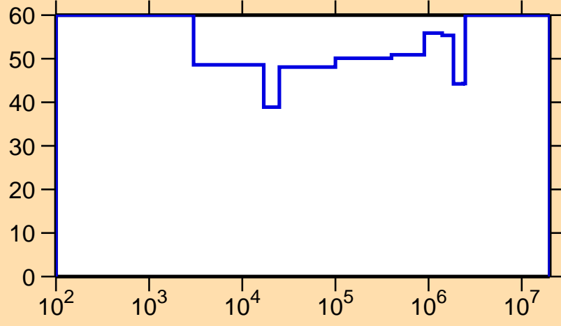
\Delta\sigma/\sigma vs. E for ^{146}\text{Eu}(n,\gamma)
