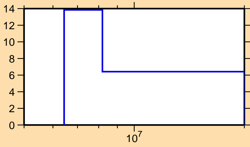
\Delta\sigma/\sigma vs. E for ^{146}\text{Eu}(n,\text{el.})
