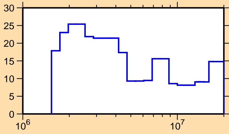
\Delta\sigma/\sigma vs. E for ^{147}\text{Eu}(n,\text{el.})
