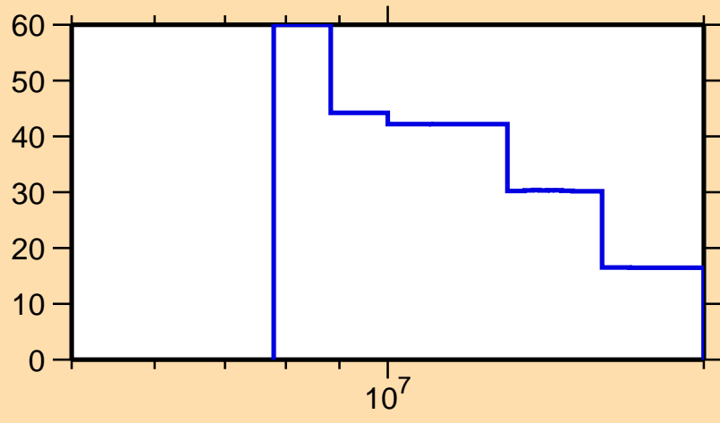
\Delta\sigma/\sigma vs. E for ^{147}\text{Eu}(n,2n)
