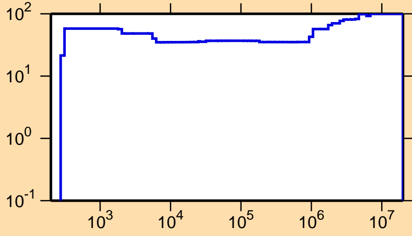
\Delta\sigma/\sigma vs. E for ^{147}\text{Eu}(n,\gamma)
