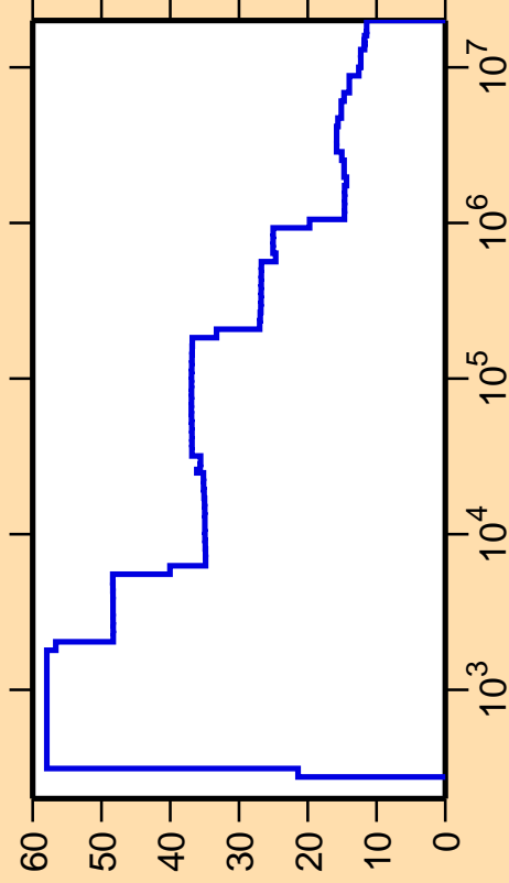
\Delta\sigma/\sigma vs. E for ^{147}\text{Eu}(n,\text{nonel.})
