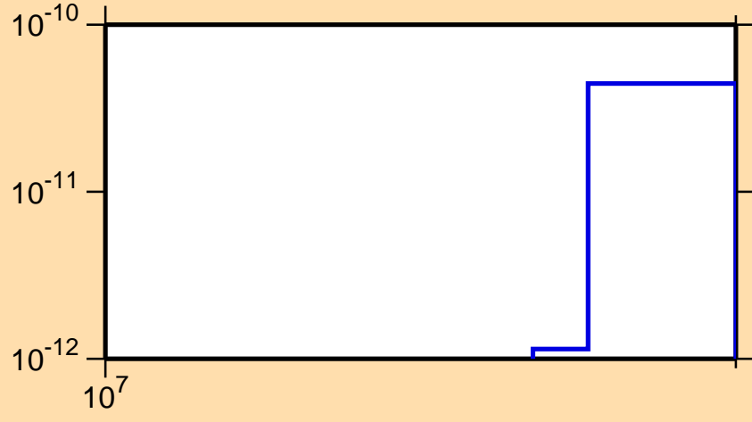
\sigma vs. E for ^{147}\text{Eu}(n,\text{pd})
