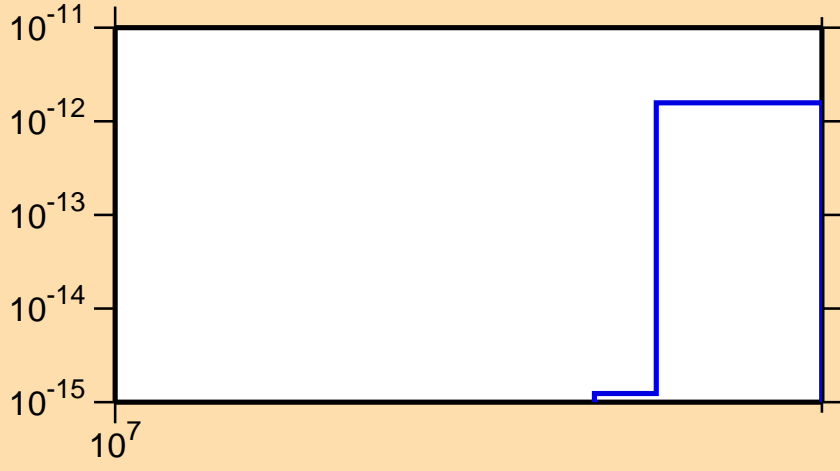
\sigma vs. E for ^{147}\text{Eu}(n,pt)
