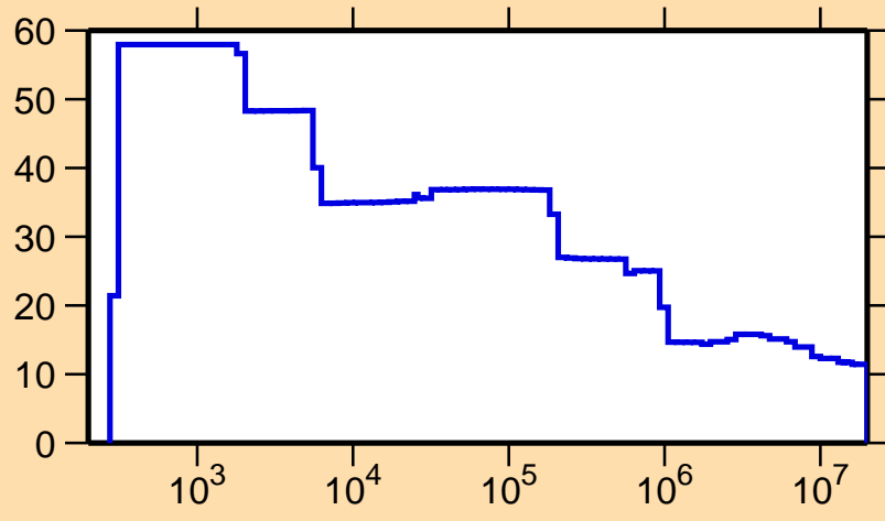
\Delta\sigma/\sigma vs. E for ^{147}\text{Eu}(n,\text{nonel.})
