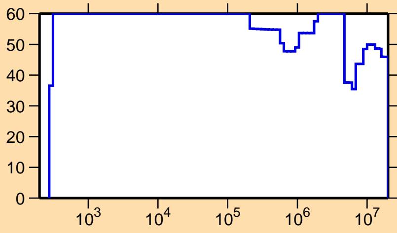
\Delta\sigma/\sigma vs. E for ^{147}\text{Eu}(n,p)
