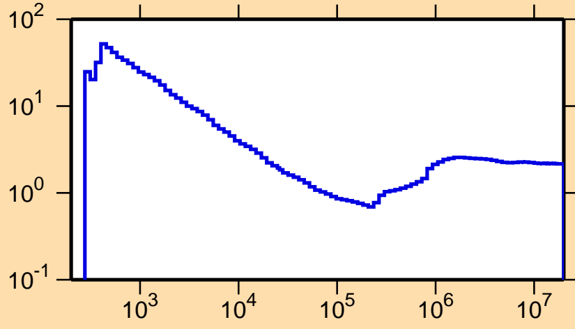
\sigma vs. E for ^{147}\text{Eu}(n,\text{nonel.})
