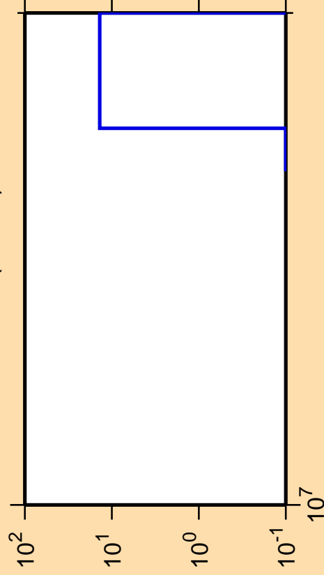
\Delta\sigma/\sigma vs. E for ^{147}\text{Eu} (mt 34)
