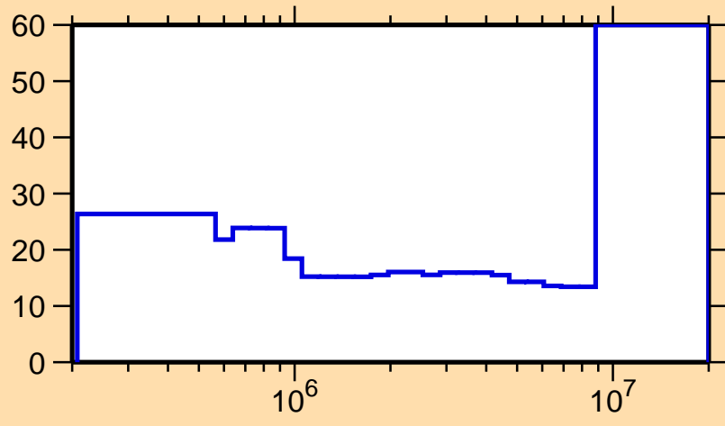
\Delta\sigma/\sigma vs. E for ^{147}\text{Eu}(n,\text{inel.})
