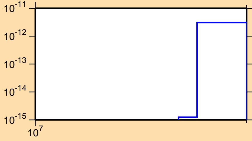
\sigma vs. E for ^{147}\text{Eu} (mt 34)
