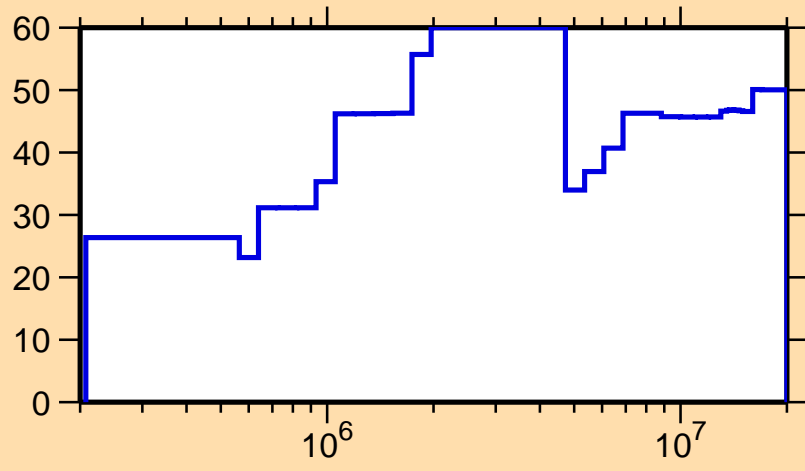
\Delta\sigma/\sigma vs. E for ^{147}\text{Eu}(n,n_1)
