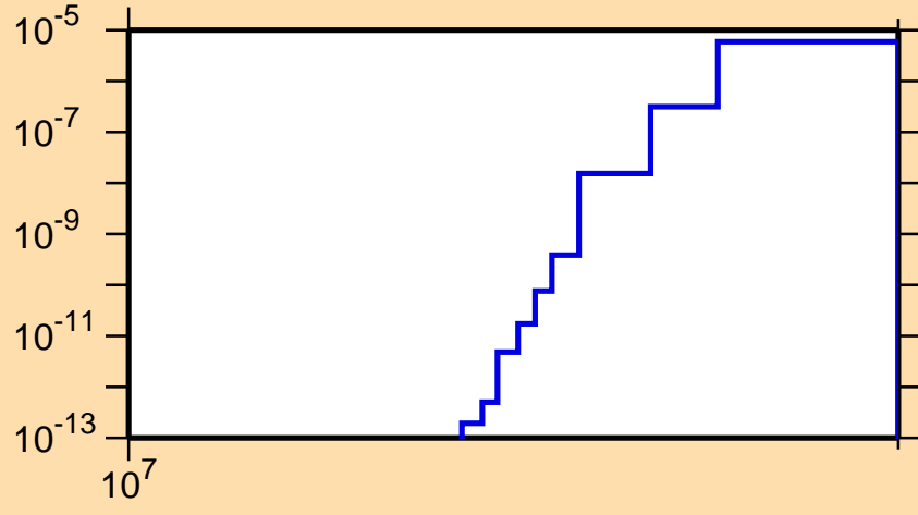
\sigma vs. E for ^{147}\text{Eu}(n,nt)
