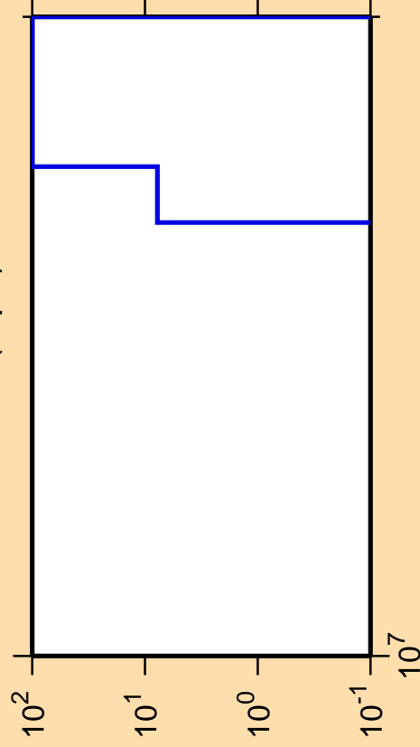
\Delta\sigma/\sigma vs. E for ^{147}\text{Eu}(n,\text{pd})
