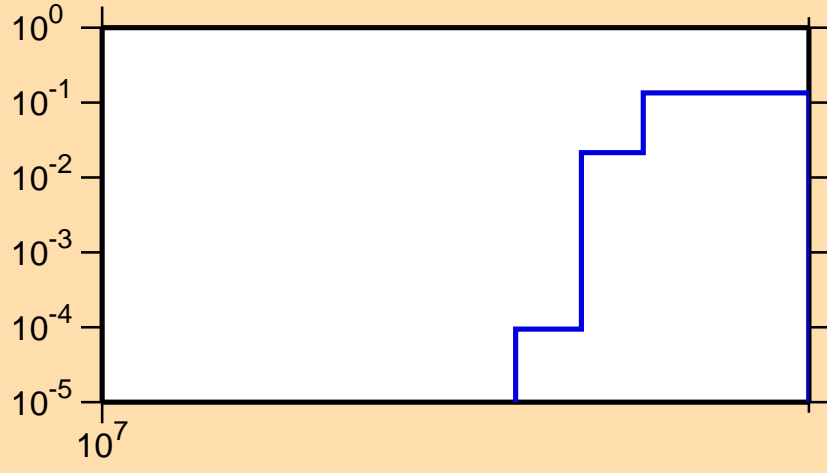
\sigma vs. E for ^{147}\text{Eu}(n,3n)
