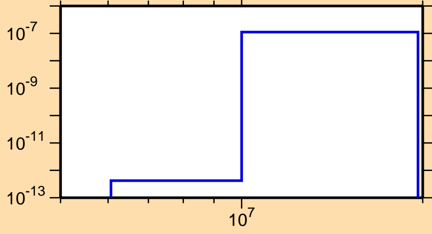
\sigma vs. E for ^{147}\text{Eu}(\text{mt } 45)
