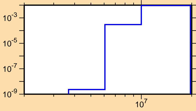
\sigma vs. E for ^{147}\text{Eu}(n,np)
