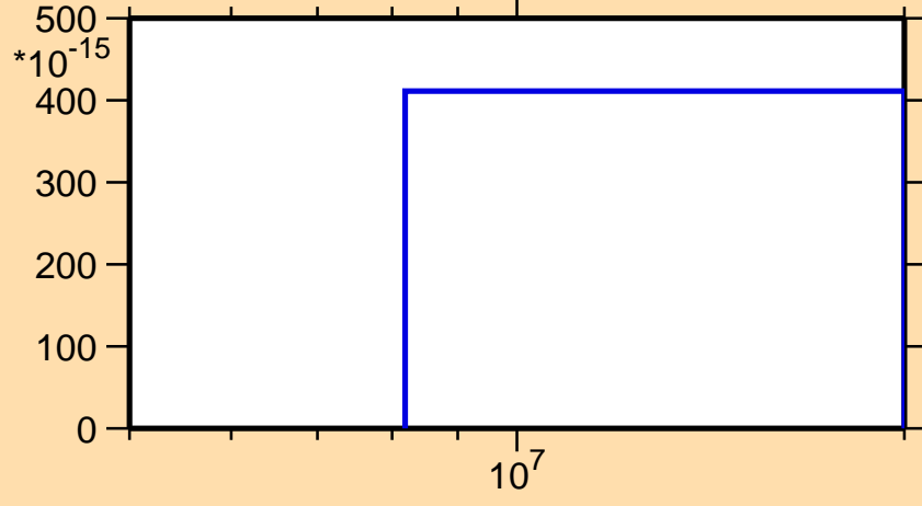
\sigma vs. E for ^{147}\text{Eu}(n,pd)
