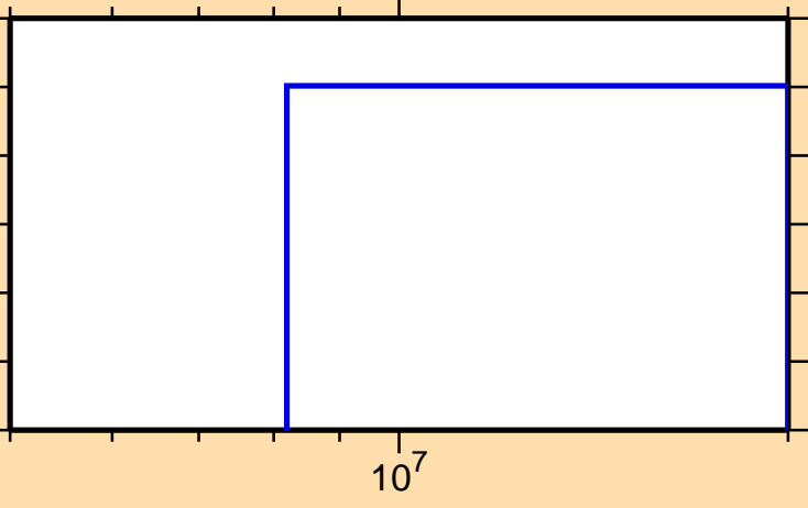
\sigma vs. E for ^{147}\text{Eu} (mt 34)
