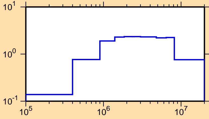
\sigma vs. E for ^{147}\text{Eu}(n,\text{inel.})
