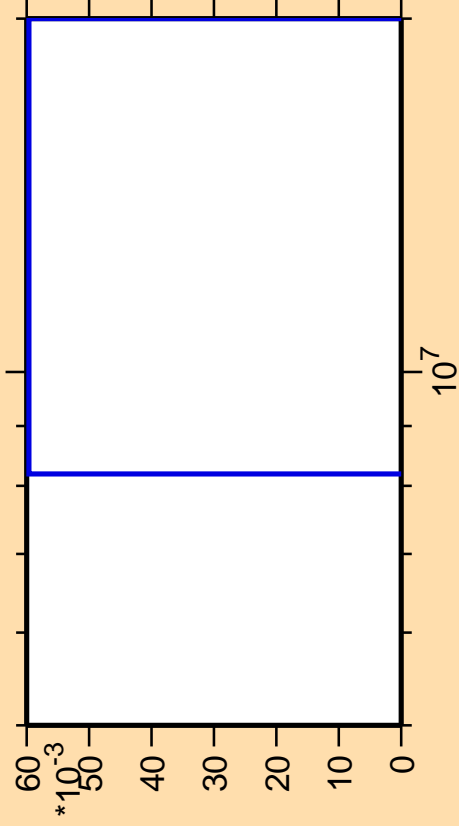
\Delta\sigma/\sigma vs. E for ^{147}\text{Eu}(n,\text{pt})
