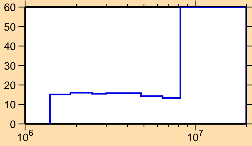
\Delta\sigma/\sigma vs. E for ^{147}\text{Eu}(n,inel.)
