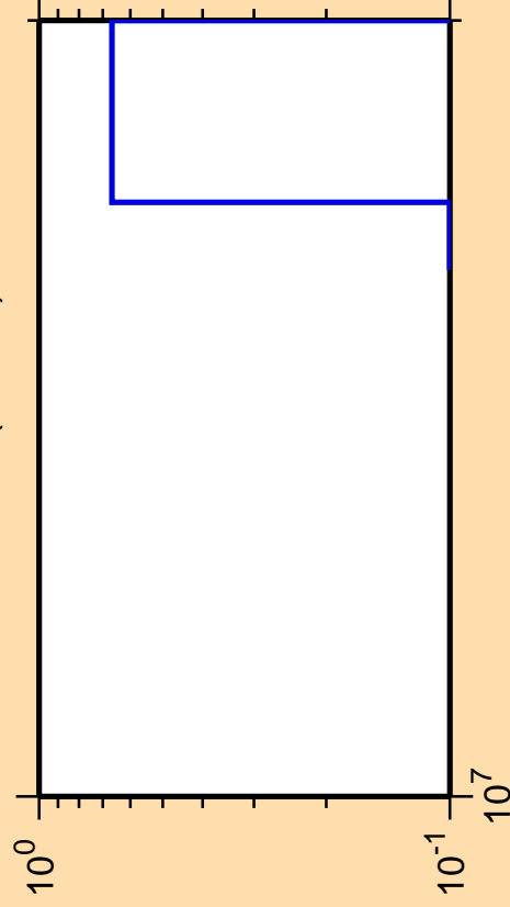
\Delta\sigma/\sigma vs. E for ^{148}\text{Eu}(n,3n\alpha)
