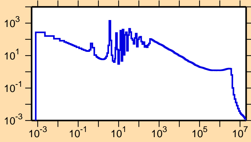
\sigma vs. E for ^{148}\text{Eu}(n,\gamma)
