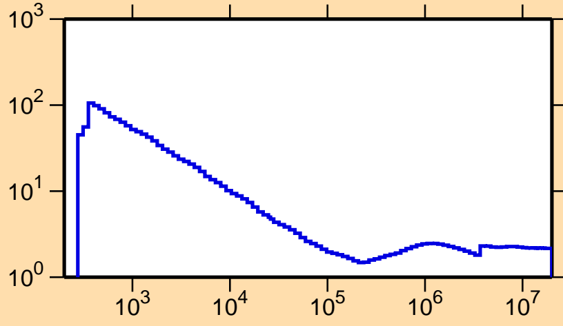
\sigma vs. E for ^{148}\text{Eu}(n,\text{nonel.})
