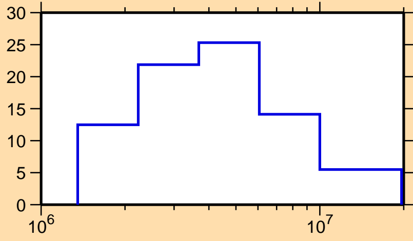
\Delta\sigma/\sigma vs. E for ^{148}\text{Eu}(n,el.)
