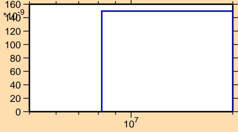
\sigma vs. E for ^{148}\text{Eu}(n,nt)
