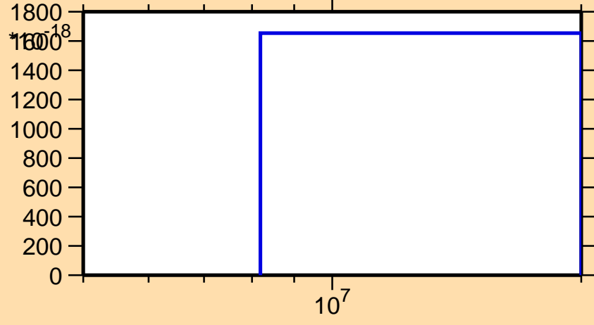
\sigma vs. E for ^{148}\text{Eu}(n,3n\alpha)
