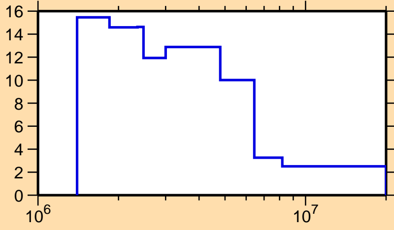
\Delta\sigma/\sigma vs. E for ^{148}\text{Eu}(n,\text{tot.})
