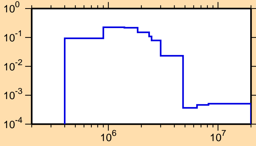
\sigma vs. E for ^{148}\text{Eu}(n,n_3)
