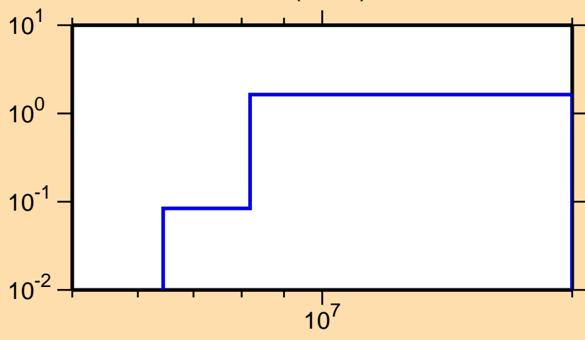
\sigma vs. E for ^{148}\text{Eu}(n,2n)
