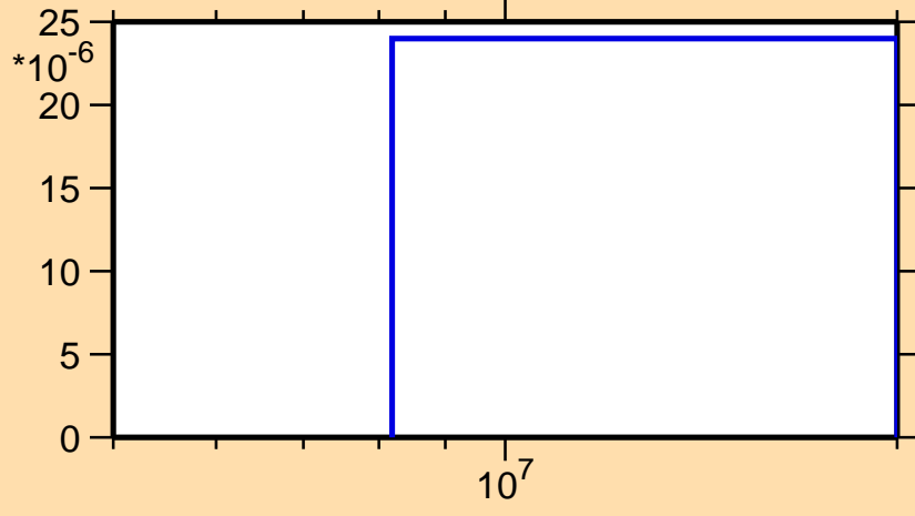
\sigma vs. E for ^{148}\text{Eu}(n,2np)
