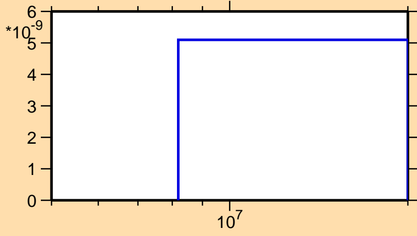
\sigma vs. E for ^{148}\text{Eu} (mt 45)
