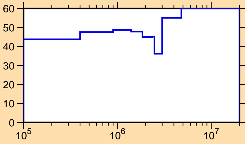
\Delta\sigma/\sigma vs. E for ^{148}\text{Eu}(n,n_1)
