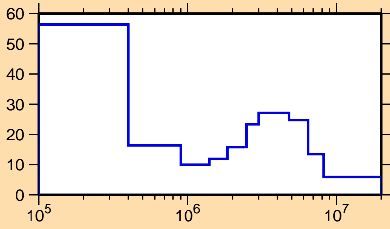
\Delta\sigma/\sigma vs. E for ^{148}\text{Eu}(n,\text{el.})
