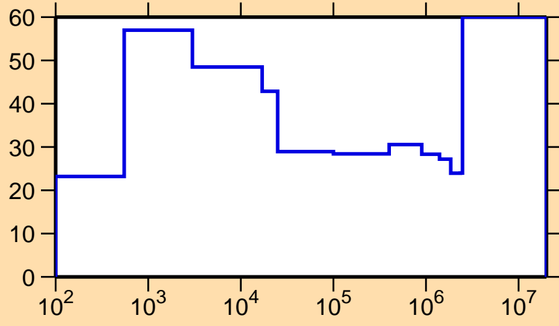
\Delta\sigma/\sigma vs. E for ^{148}\text{Eu}(n,\gamma)
