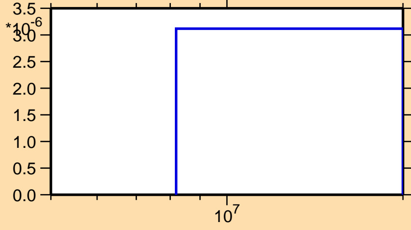
\sigma vs. E for ^{148}\text{Eu}(n,nd)
