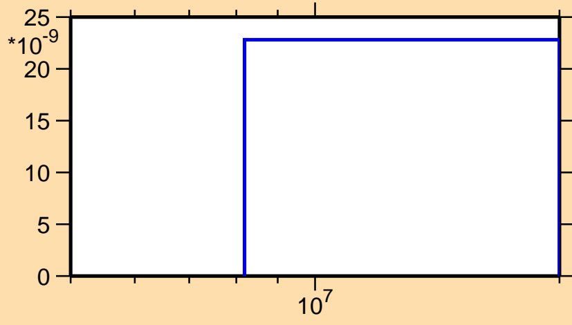
\sigma vs. E for ^{148}\text{Eu}(n,\text{He}3)
