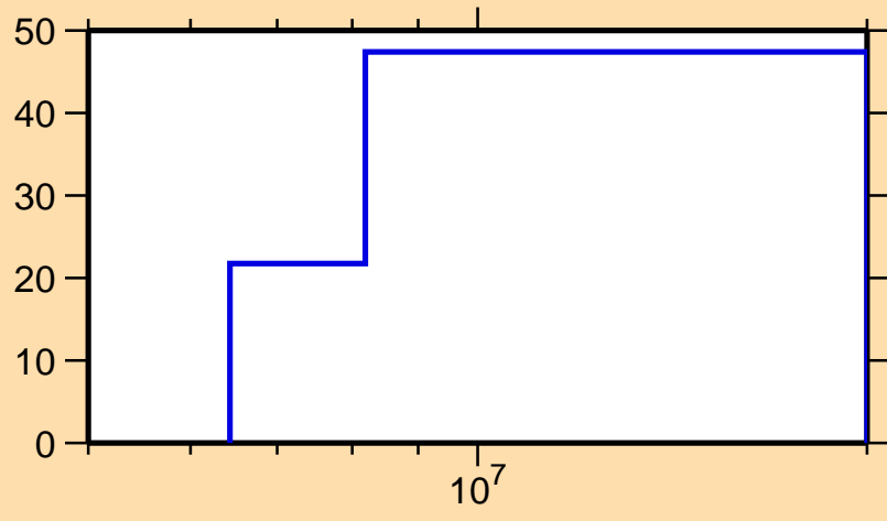
\Delta\sigma/\sigma vs. E for ^{148}\text{Eu}(n,\text{inel.})
