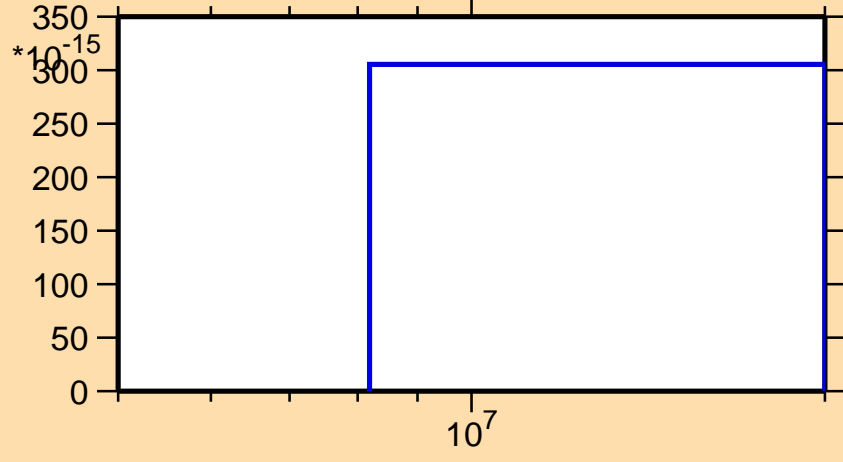
\sigma vs. E for ^{148}\text{Eu}(\text{mt } 34)
