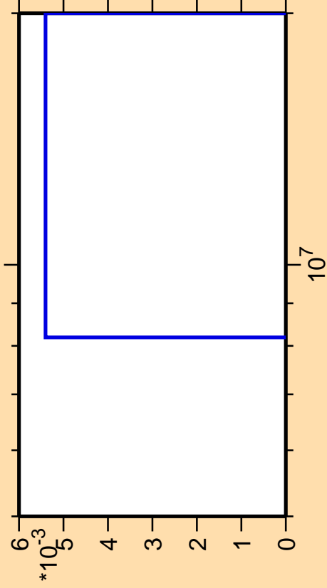
\Delta\sigma/\sigma vs. E for ^{148}\text{Eu}(n,3n\alpha)
