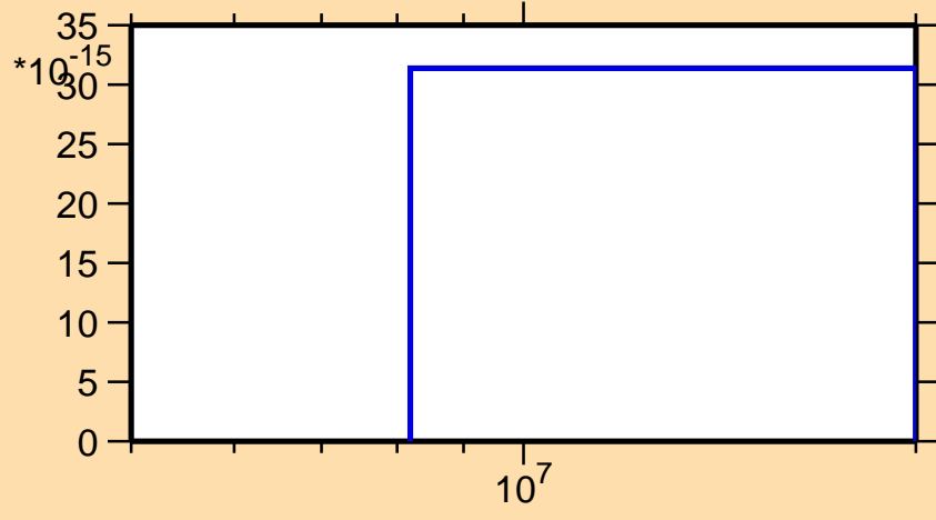
\sigma vs. E for ^{148}\text{Eu}(n,pd)
