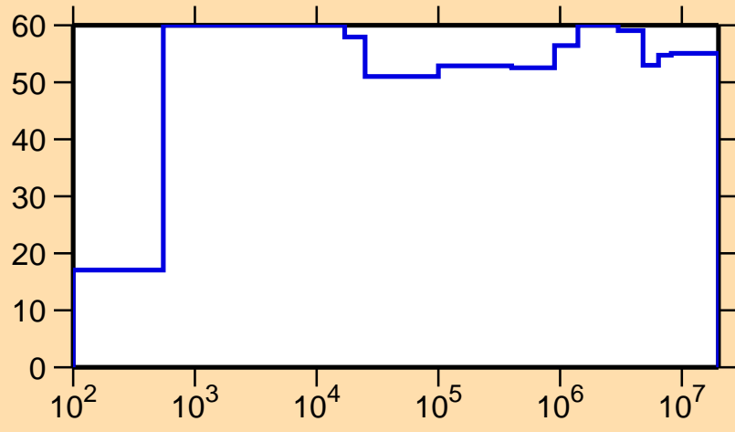
\Delta\sigma/\sigma vs. E for ^{148}\text{Eu}(n,p)
