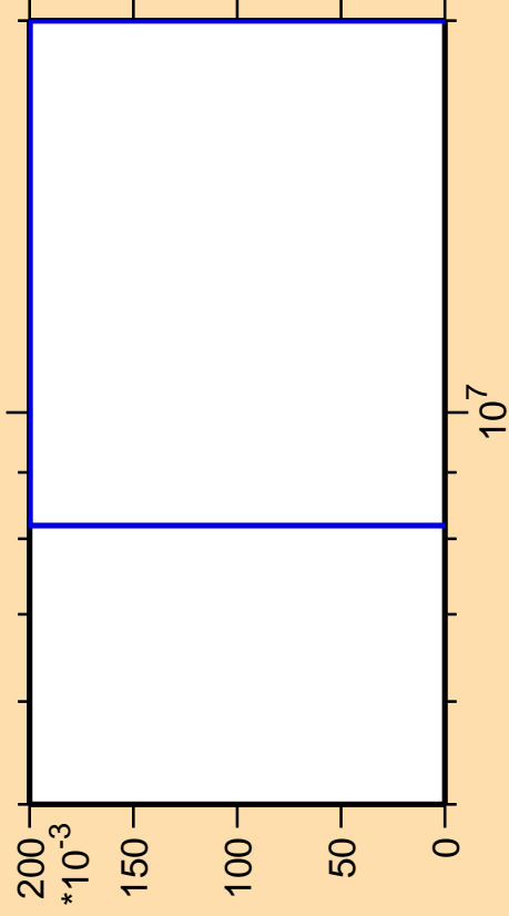
\Delta\sigma/\sigma vs. E for ^{148}\text{Eu}(n,pd)
