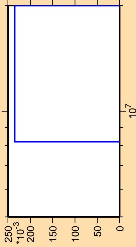
\Delta\sigma/\sigma vs. E for ^{148}\text{Eu}(n,pt)
