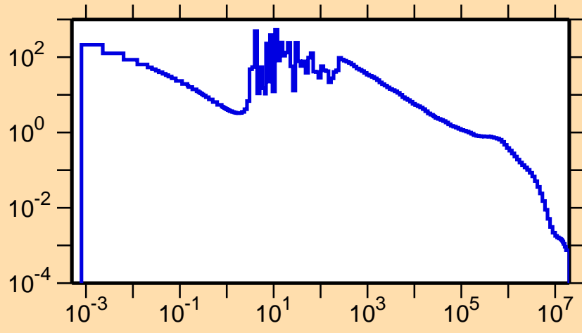
\sigma vs. E for ^{149}\text{Eu}(n,\gamma)
