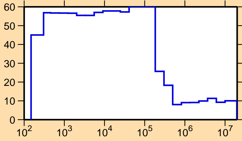
\Delta\sigma/\sigma vs. E for ^{149}\text{Eu}(n,\text{el.})
