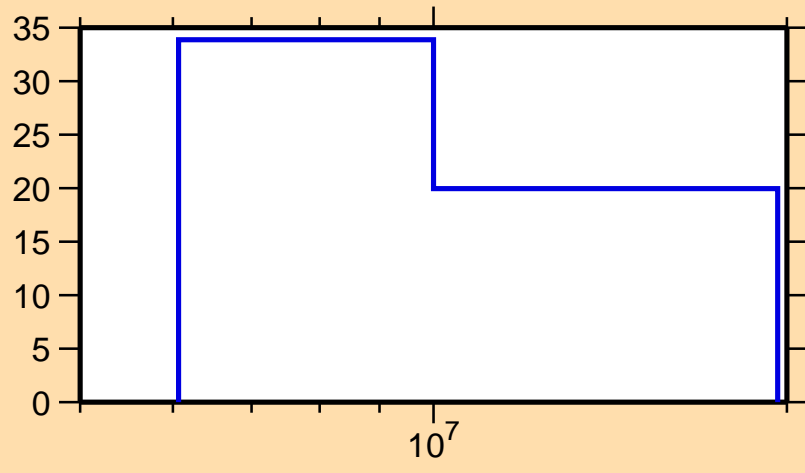
\Delta\sigma/\sigma vs. E for ^{149}\text{Eu}(n,2n)
