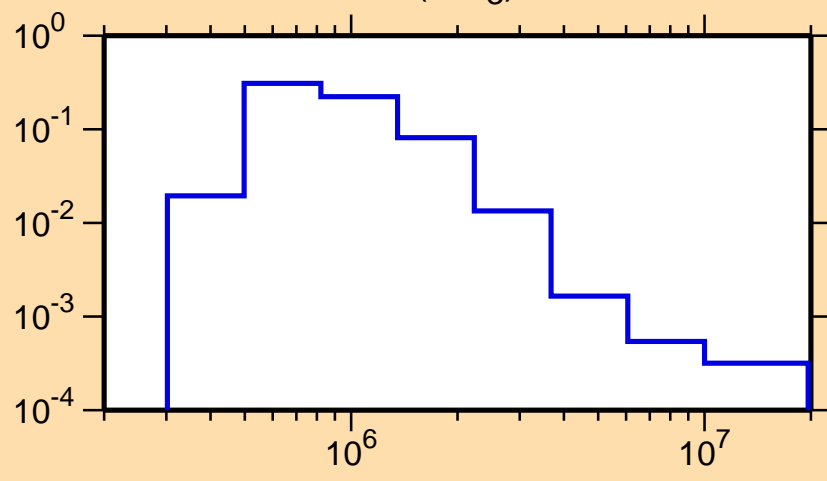
\sigma vs. E for ^{149}\text{Eu}(n,n_3)
