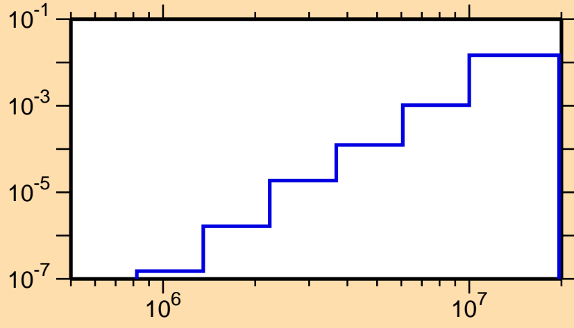
\sigma vs. E for ^{149}\text{Eu}(n,p)
