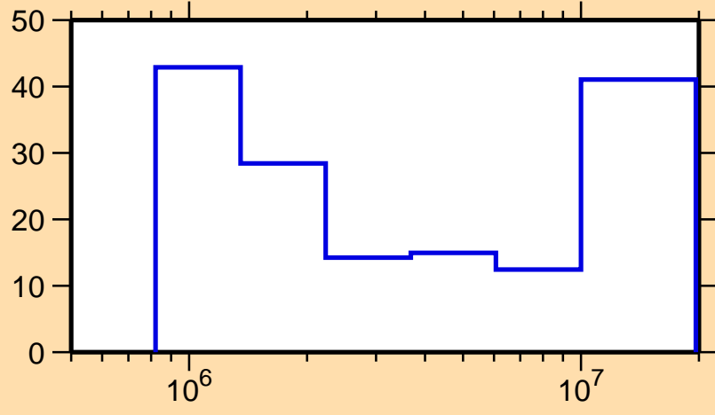
\Delta\sigma/\sigma vs. E for ^{149}\text{Eu}(n,n\text{cont.})
