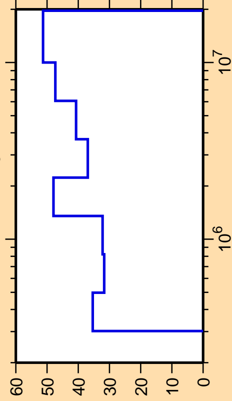
\Delta\sigma/\sigma vs. E for ^{149}\text{Eu}(n,n_3)
