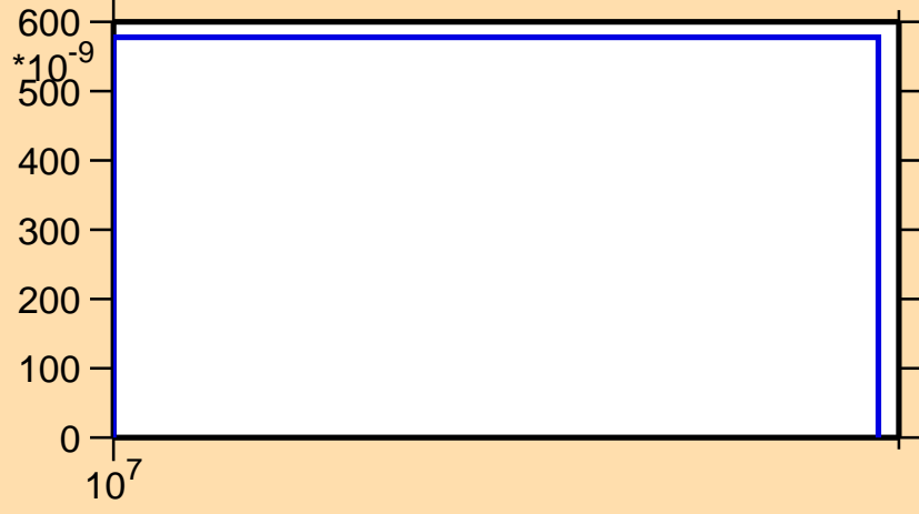
\sigma vs. E for ^{149}\text{Eu}(n,\text{nd})
