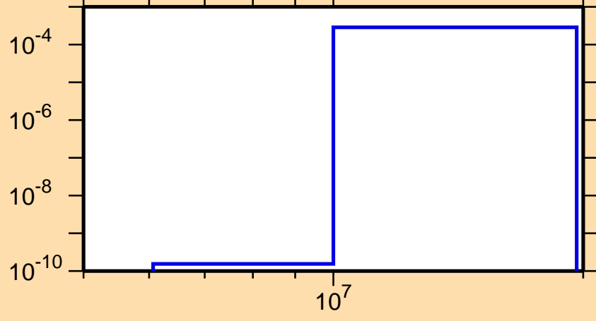
\sigma vs. E for ^{149}\text{Eu}(n,t)
