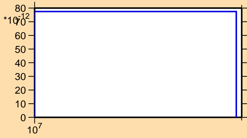
\sigma vs. E for ^{149}\text{Eu}(n,3n\alpha)
