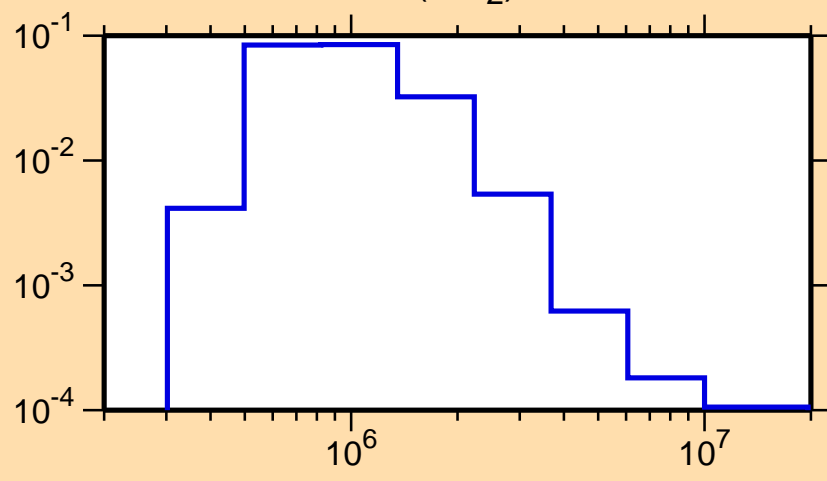
\sigma vs. E for ^{149}\text{Eu}(n,n_2)
