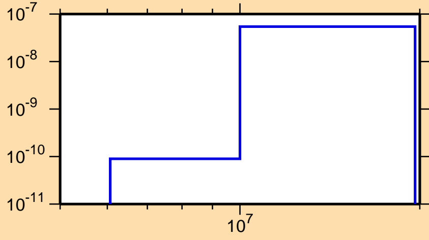
\sigma vs. E for ^{149}\text{Eu}(n,p\alpha)
