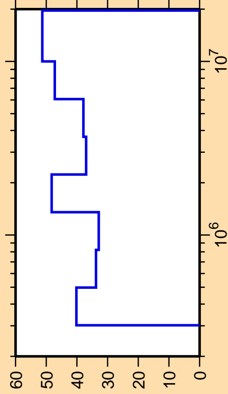
\Delta\sigma/\sigma vs. E for ^{149}\text{Eu}(n,n_2)
