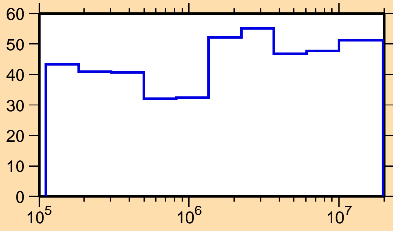
\Delta\sigma/\sigma vs. E for ^{149}\text{Eu}(n,n_1)
