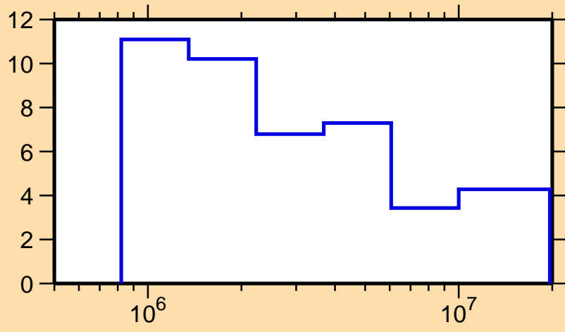
\Delta\sigma/\sigma vs. E for ^{149}\text{Eu}(n,\text{tot.})
