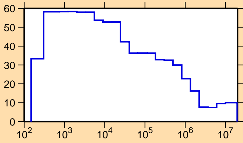
\Delta\sigma/\sigma vs. E for ^{149}\text{Eu}(n,\text{nonel.})
