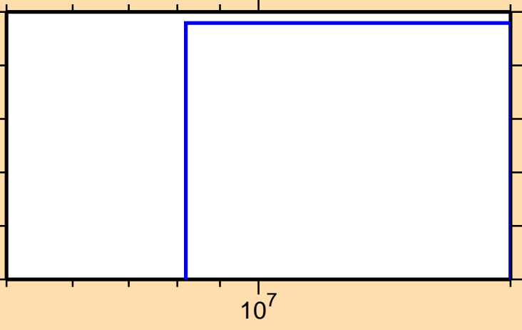
\sigma vs. E for ^{149}\text{Eu}(n,nd)
