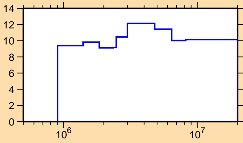
\Delta\sigma/\sigma vs. E for ^{149}\text{Eu}(n, el.)
