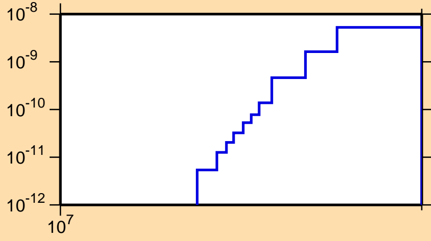
\sigma vs. E for ^{150}\text{Eu}(\text{mt117})
