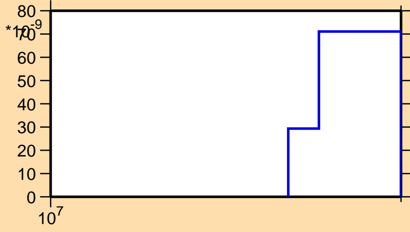
\sigma vs. E for ^{150}\text{Eu}(n,3n\alpha)
