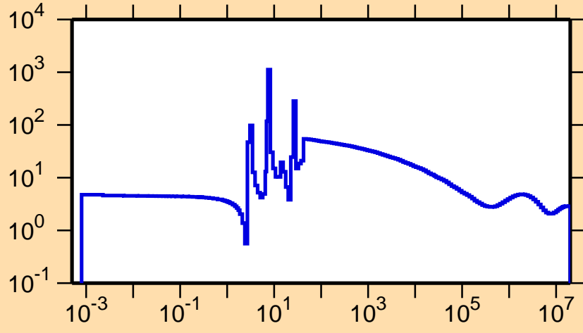
\sigma vs. E for ^{150}\text{Eu}(n,\text{el.})
