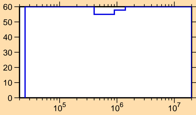
\Delta\sigma/\sigma vs. E for ^{150}\text{Eu}(n,n_1)
