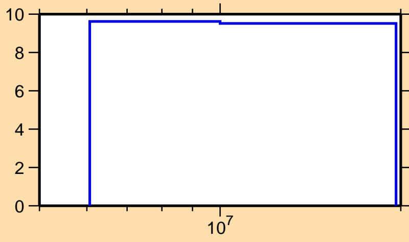
\Delta\sigma/\sigma vs. E for ^{150}\text{Eu}(n,2n)
