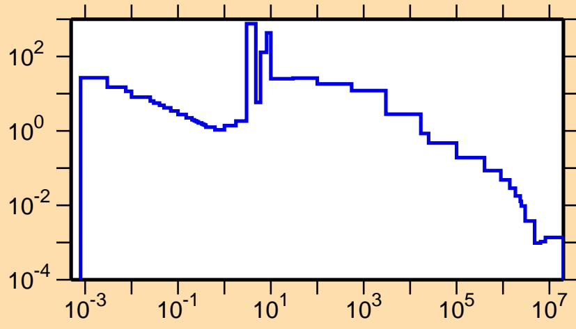
\sigma vs. E for ^{150}\text{Eu}(n,\gamma)
