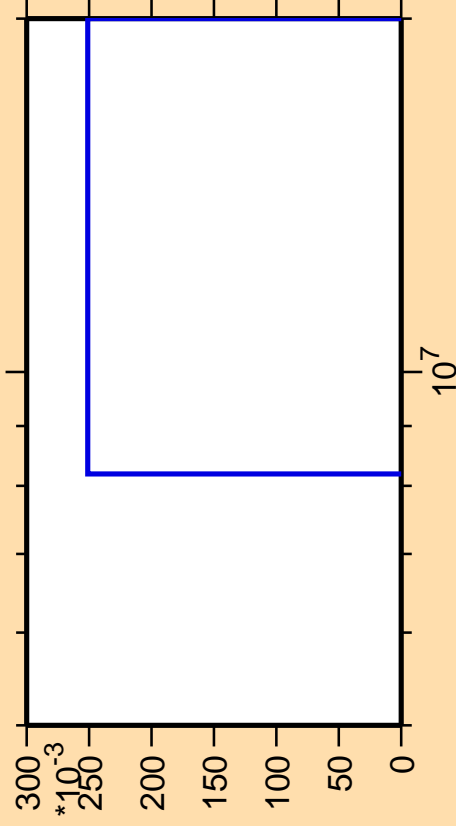
\Delta\sigma/\sigma vs. E for ^{150}\text{Eu}(\text{mt } 34)
