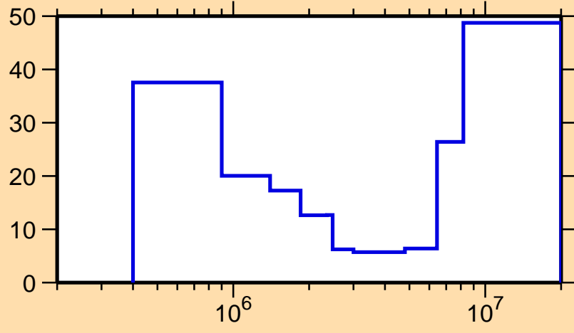
\Delta\sigma/\sigma vs. E for ^{150}\text{Eu}(n,n\text{cont.})
