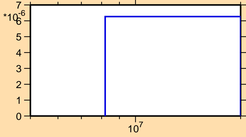
\sigma vs. E for ^{150}\text{Eu}(n,nd)
