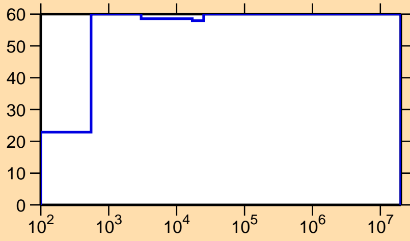
\Delta\sigma/\sigma vs. E for ^{150}\text{Eu}(n,\gamma)
