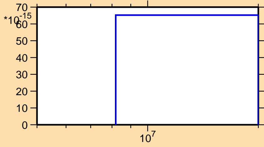
\sigma vs. E for ^{150}\text{Eu}(\text{mt } 34)
