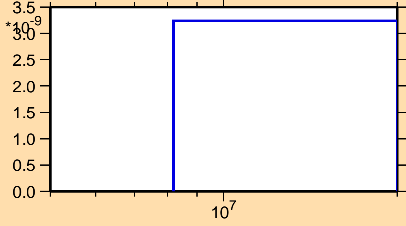
\sigma vs. E for ^{150}\text{Eu}(n,\text{He}3)
