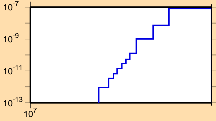
\sigma vs. E for ^{151}\text{Eu}(n,\text{He3})
