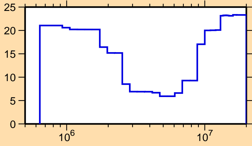
\Delta\sigma/\sigma vs. E for ^{151}\text{Eu}(n,n\text{cont.})
