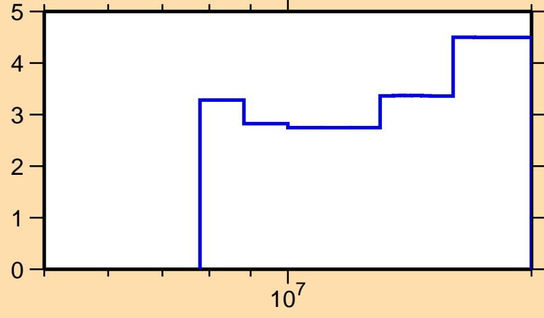
\Delta\sigma/\sigma vs. E for ^{151}\text{Eu}(n,\text{tot.})
