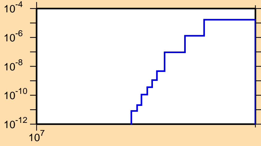
\sigma vs. E for ^{151}\text{Eu}(n,nd)
