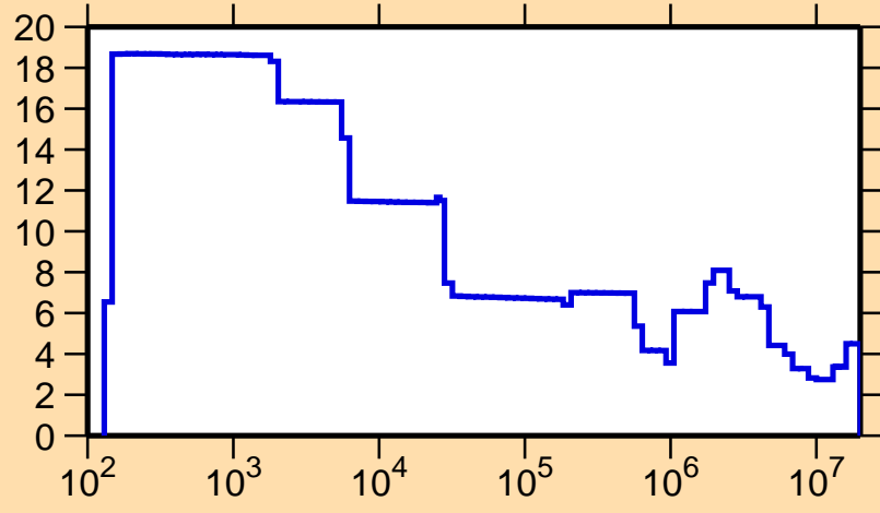
\Delta\sigma/\sigma vs. E for ^{151}\text{Eu}(n,\text{tot.})
