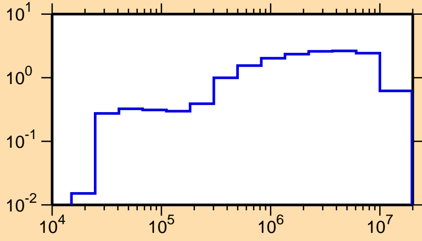
\sigma vs. E for ^{151}\text{Eu}(n,\text{inel.})
