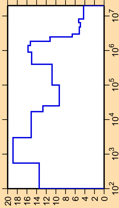
\Delta\sigma/\sigma vs. E for ^{151}\text{Eu}(n,\text{nonel.})
