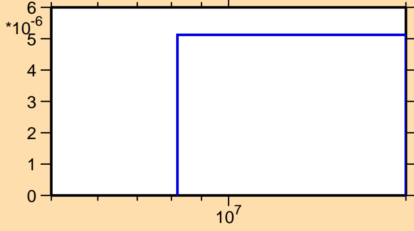
\sigma vs. E for ^{151}\text{Eu}(n,2n\alpha)
