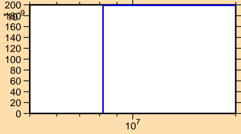
\sigma vs. E for ^{151}\text{Eu}(n,nd)
