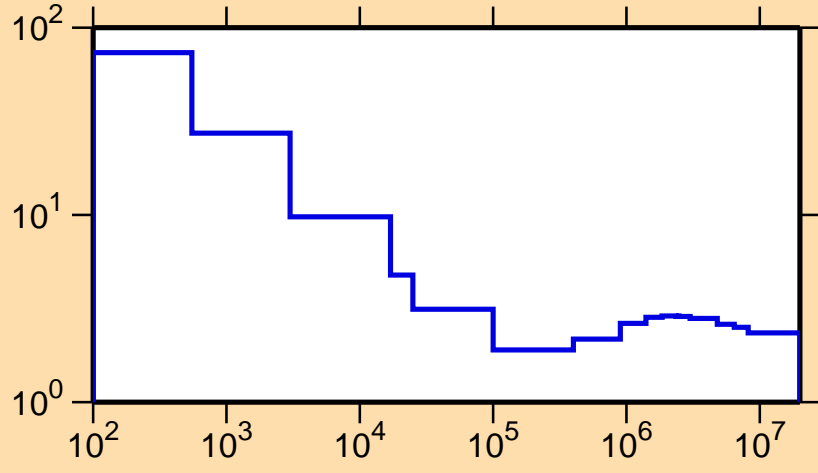
\sigma vs. E for ^{151}\text{Eu}(n,\text{nonel.})
