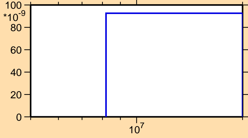
\sigma vs. E for ^{151}\text{Eu}(n,2np)
