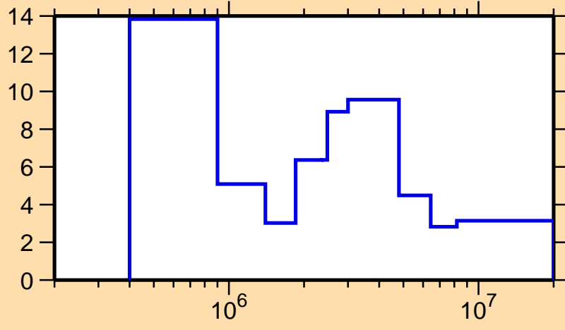
\Delta\sigma/\sigma vs. E for ^{151}\text{Eu}(n, el.)
