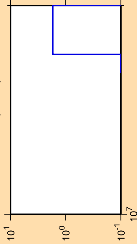
\Delta\sigma/\sigma vs. E for ^{152}\text{Eu} (mt 34)
