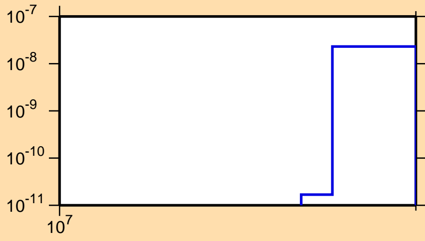
\sigma vs. E for ^{152}\text{Eu}(n,3n\alpha)
