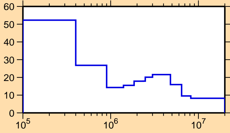
\Delta\sigma/\sigma vs. E for ^{152}\text{Eu}(n, el.)
