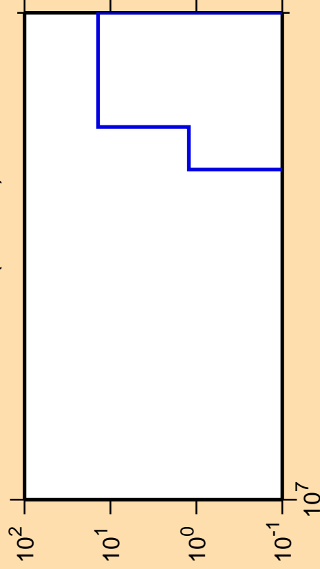
\Delta\sigma/\sigma vs. E for ^{153}\text{Eu}(\text{mt117})
