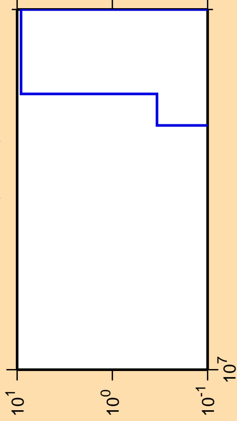
\Delta\sigma/\sigma vs. E for ^{153}\text{Eu} (mt 45)
