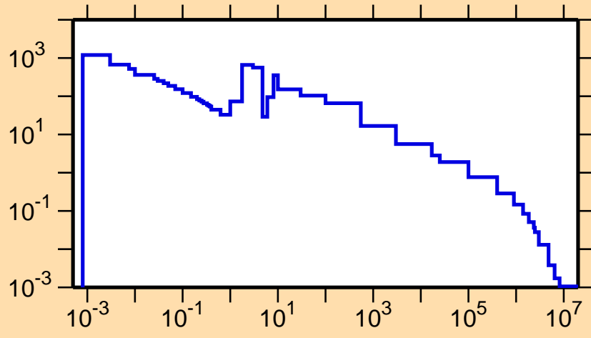
\sigma vs. E for ^{153}\text{Eu}(n,\gamma)
