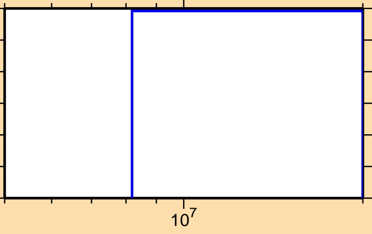
\sigma vs. E for ^{153}\text{Eu}(n,2np)
