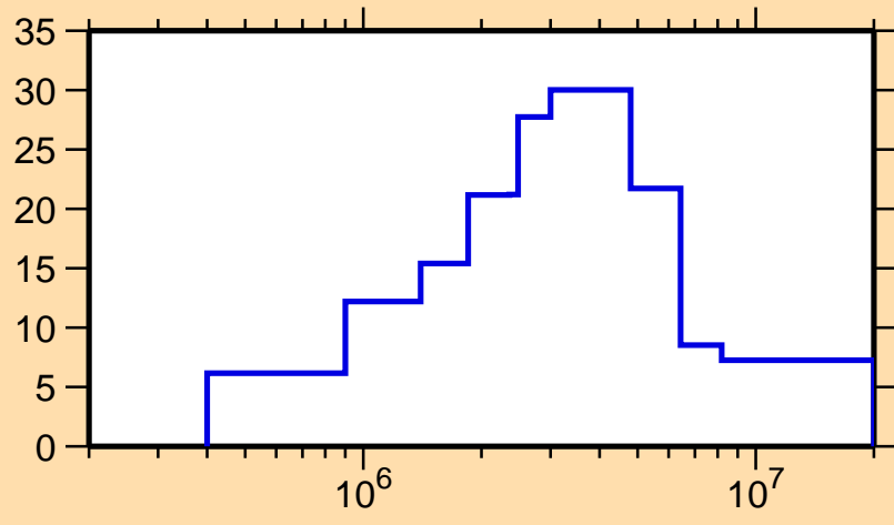
\Delta\sigma/\sigma vs. E for ^{153}\text{Eu}(n, el.)
