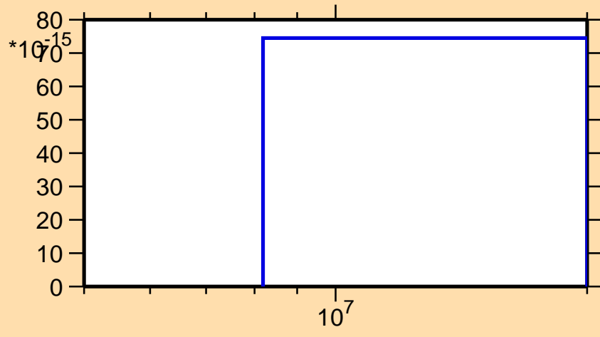
\sigma vs. E for ^{153}\text{Eu}(n,3n\alpha)
