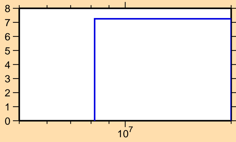
\Delta\sigma/\sigma vs. E for ^{153}\text{Eu}(n,\text{el.})
