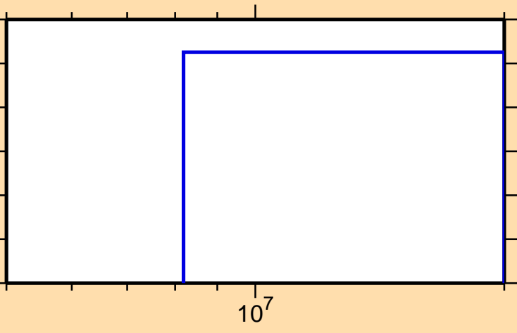
\sigma vs. E for ^{153}\text{Eu}(n,\text{He3})
