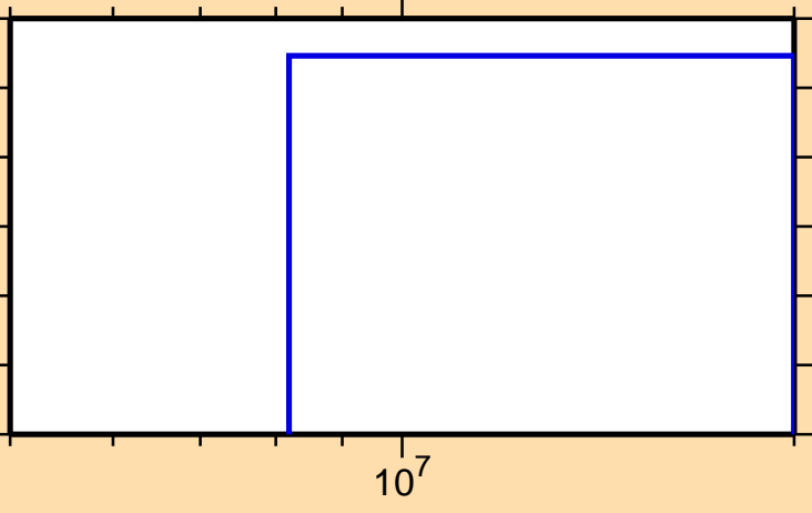
\sigma vs. E for ^{153}\text{Eu}(n,t)
