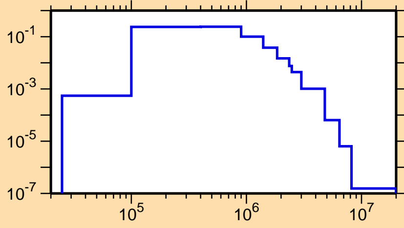
\sigma vs. E for ^{153}\text{Eu}(n,n_2)
