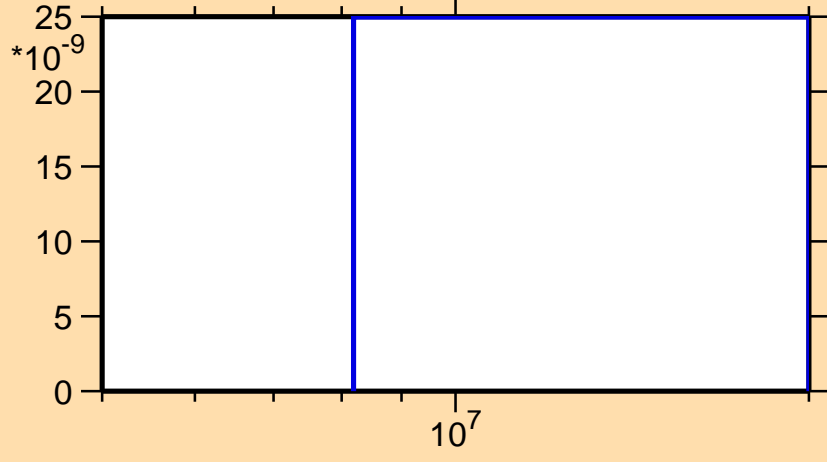
\sigma vs. E for ^{153}\text{Eu}(n,nd)
