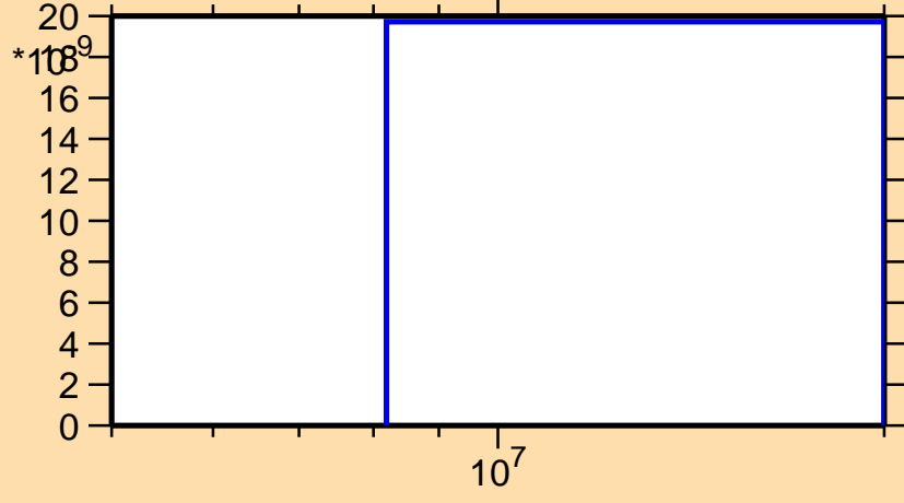
\sigma vs. E for ^{153}\text{Eu}(n,nt)
