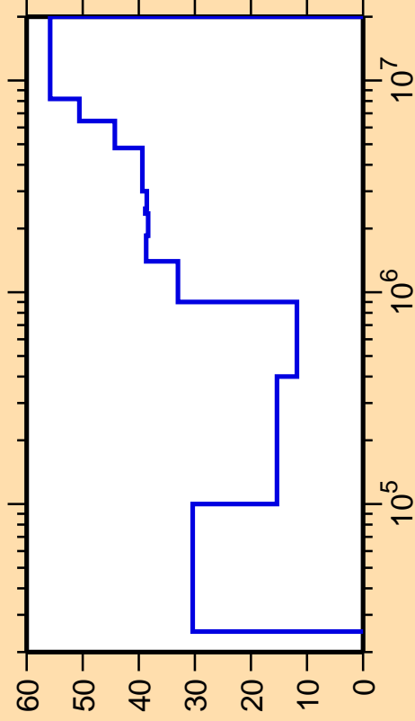
\Delta\sigma/\sigma vs. E for ^{153}\text{Eu}(n,n_2)
