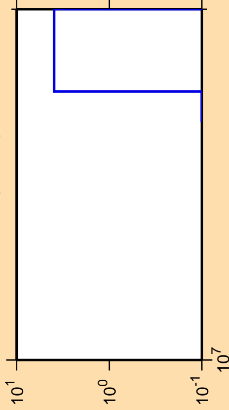
\Delta\sigma/\sigma vs. E for ^{154}\text{Eu}(n,3n\alpha)
