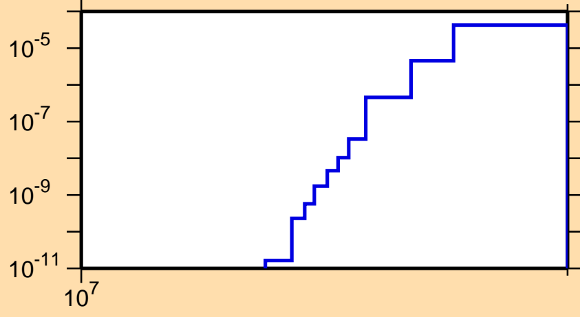
\sigma vs. E for ^{154}\text{Eu}(n,nd)
