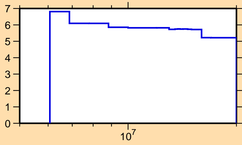
\Delta\sigma/\sigma vs. E for ^{154}\text{Eu}(n,\text{nonel.})
