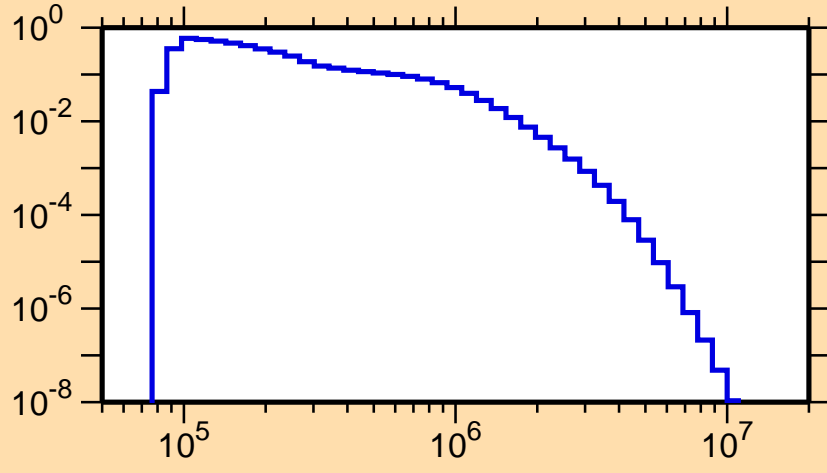
\sigma vs. E for ^{154}\text{Eu}(n,n_3)
