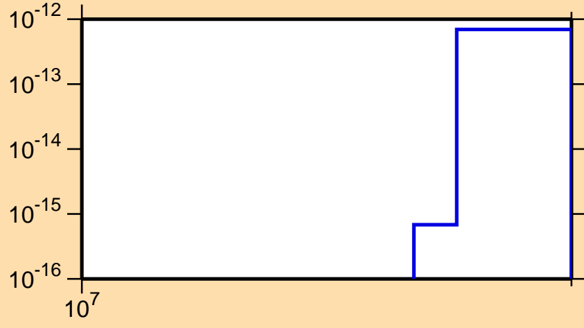
\sigma vs. E for ^{154}\text{Eu}(n,3n\alpha)
