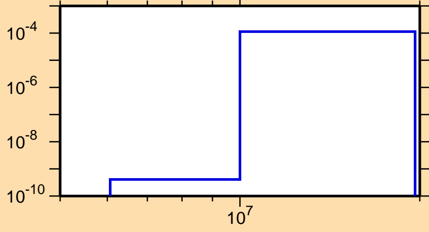
\sigma vs. E for ^{154}\text{Eu}(n,t)
