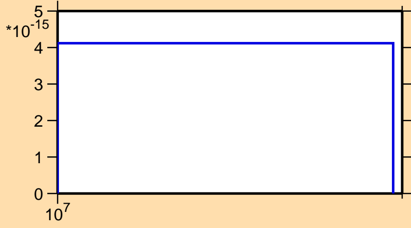
\sigma vs. E for ^{154}\text{Eu}(n,3n\alpha)
