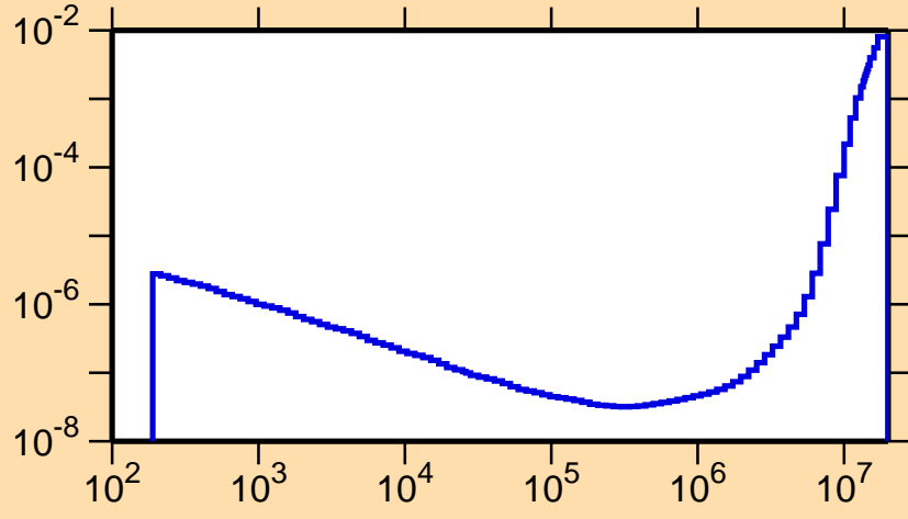
\sigma vs. E for ^{154}\text{Eu}(n,\alpha)
