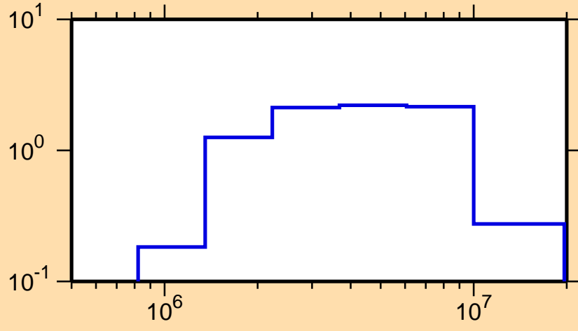
\sigma vs. E for ^{155}\text{Eu}(n,n\text{cont.})
