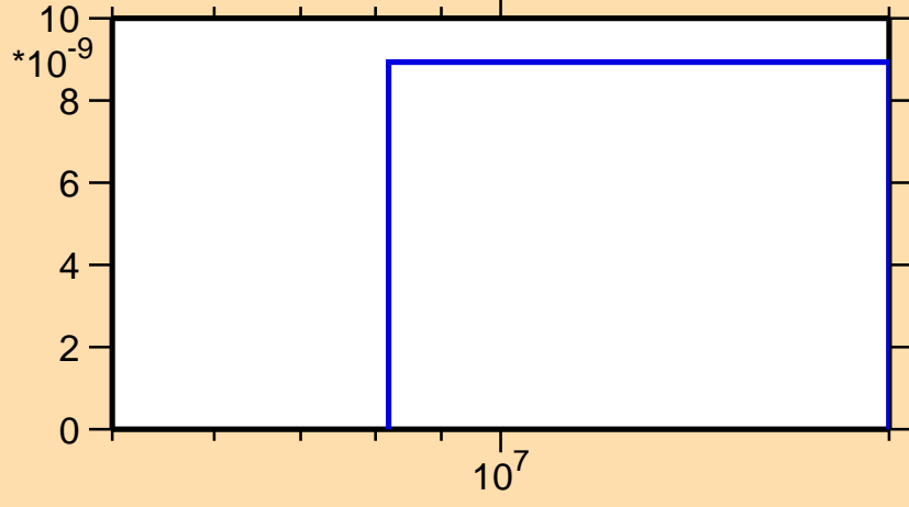
\sigma vs. E for ^{155}\text{Eu}(n,nd)
