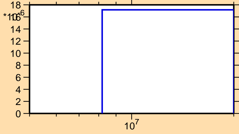
\sigma vs. E for ^{155}\text{Eu}(n,t)
