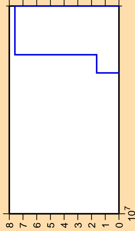
\Delta\sigma/\sigma vs. E for ^{156}\text{Eu}(n,p\alpha)
