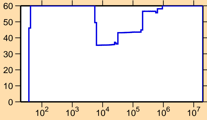
\Delta\sigma/\sigma vs. E for ^{156}\text{Eu}(n,\gamma)
