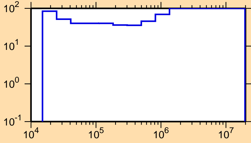
\Delta\sigma/\sigma vs. E for ^{156}\text{Eu}(n,n_1)
