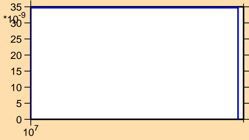
\sigma vs. E for ^{156}\text{Eu}(n,2np)
