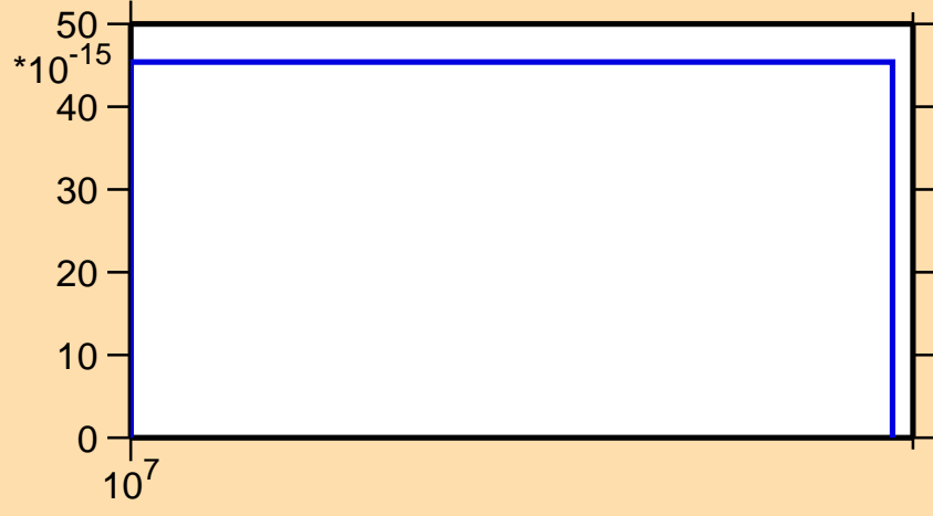
\sigma vs. E for ^{156}\text{Eu}(n,p\alpha)
