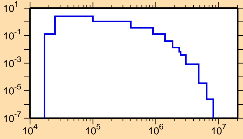
\sigma vs. E for ^{156}\text{Eu}(n,n_1)
