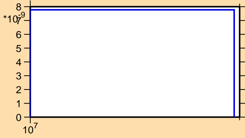
\sigma vs. E for ^{157}\text{Eu}(n,\text{nd})
