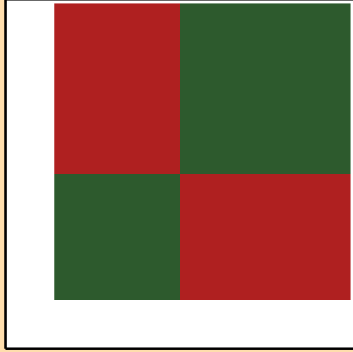
\sigma vs. E for ^{157}\text{Eu}(n,2n)
