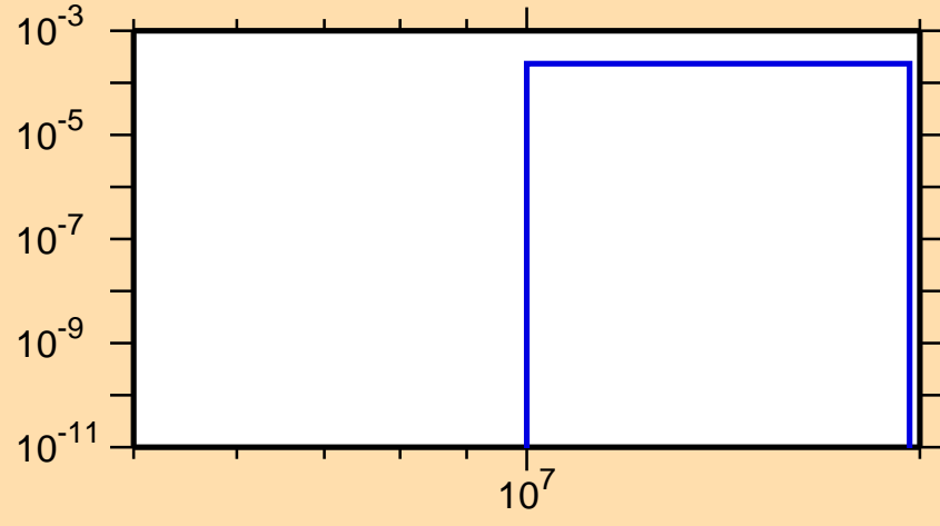
\sigma vs. E for ^{157}\text{Eu}(n,np)
