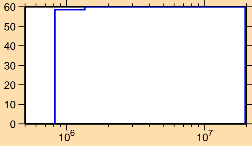
\Delta\sigma/\sigma vs. E for ^{157}\text{Eu}(n,\gamma)
