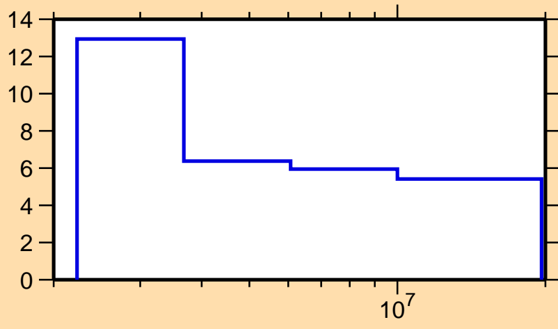
\Delta\sigma/\sigma vs. E for ^{157}\text{Eu}(n,\text{tot.})
