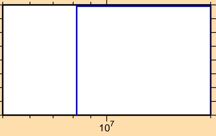
\sigma vs. E for ^{157}\text{Eu}(n,nt)
