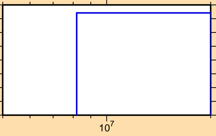
\sigma vs. E for ^{157}\text{Eu}(n,nd)
