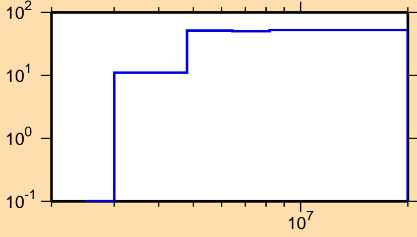
\Delta\sigma/\sigma vs. E for ^{157}\text{Eu}(n,p)
