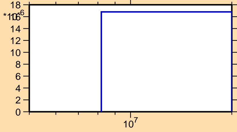
\sigma vs. E for ^{157}\text{Eu}(n,t)
