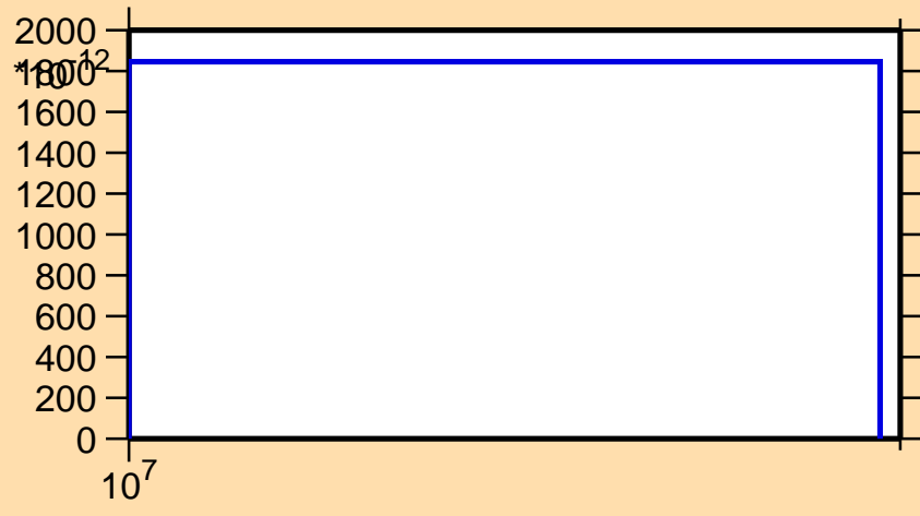
\sigma vs. E for ^{158}\text{Eu}(n,2n\alpha)
