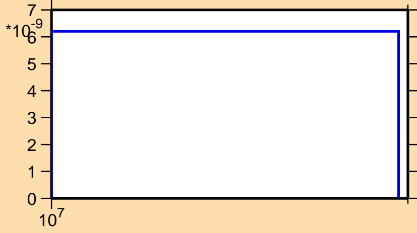
\sigma vs. E for ^{158}\text{Eu}(n,2np)
