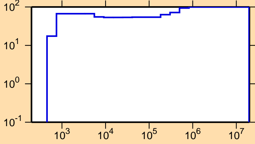
\Delta\sigma/\sigma vs. E for ^{158}\text{Eu}(n,\gamma)
