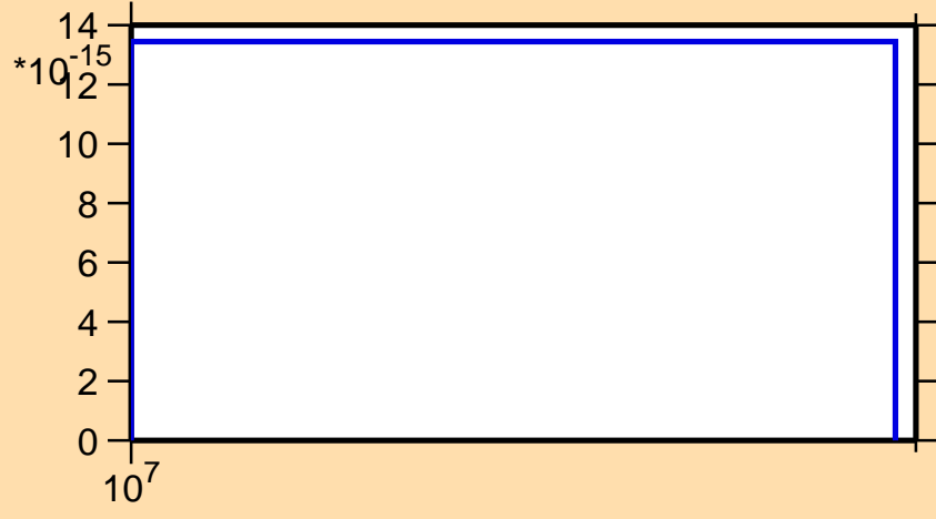
\sigma vs. E for ^{158}\text{Eu}(n,\text{He3})
